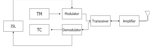
Fig. 9: ISL communications: The block diagram illustrates the Inter-satellite link communication system, including the S-band patch antenna, the amplifier, the modulator and demodulator blocks, and the Telemetry (TM) and Telecommand (TC) blocks, which are discussed in Section 8
