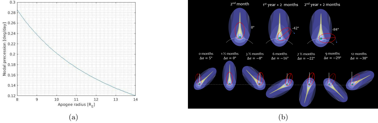
Fig. 5: Variation of nodal precession against apogee: (a) The equatorial orbit used in the mission will experience nodal precession rates of 0.12^{\circ} – 0.29^{\circ} per day while the apogee radius is 8–14 R_E . (b) Precession of the equatorial orbit relative to the magnetotail.
