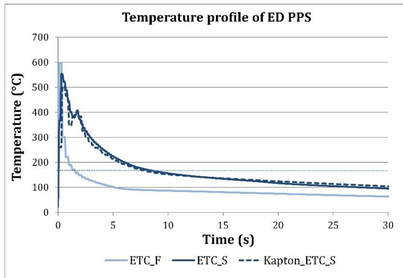
Figure 3.7. Temperature evolution during ultrasonic welding of ETC_F, ETC_S and Kapton_ETC_S. Only one specimen per series is illustrated for clarity purposes.
