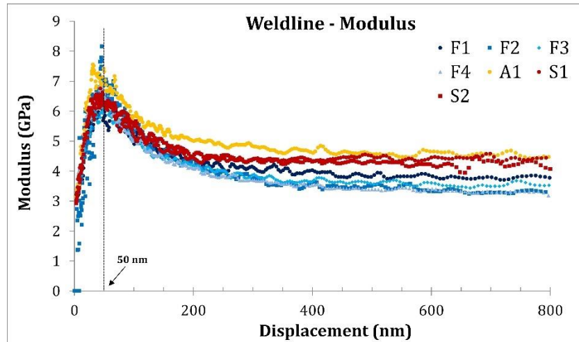
Figure 4.10. "Magnification" of Figure 4.8, showing the sharp increase of elastic modulus at shallow depths.
