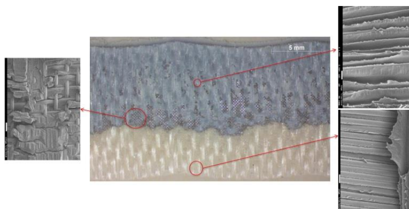
Figure 2.13. Fracture surface of specimen tested at -50 °C (centre). SEM micrographs illustrate fibre/matrix debonding (right) and mesh/ matrix debonding (left). The top right SEM image illustrates fibre imprints in the resin and the bottom right SEM image illustrates debonded fibres.
