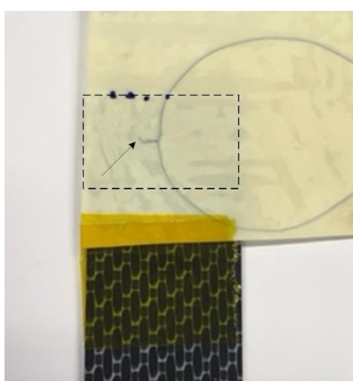
Figure 3.4. ED with embedded thermocouple prior to ultrasonic welding, positioned in such way to measure the temperature at the centre of the overlap (area enclosed within the dashed rectangle). The arrow in the picture points at the tip of the thermocouple (location of the temperature measurements).
