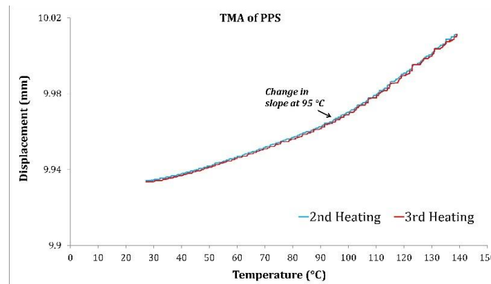
Figure 2.4. Thermal expansion of PPS as resulting from TMA tests (2 ^\circ\text{C}/\text{min} ).
