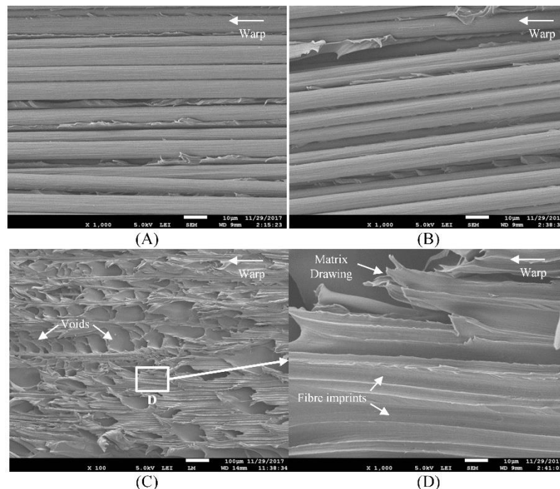
Figure 5.11. SEM micrographs of locations A-C of Figure 5.10 : (A) & (B) Extensive fibre/matrix debonding accompanied by matrix drawing. (C) Large amount of voids accompanied by ductile failure. (D) Magnification of location D of Figure 5.11C , showing substantial matrix drawing and fibre imprints. The arrow at the top right of each image indicates the warp direction.
