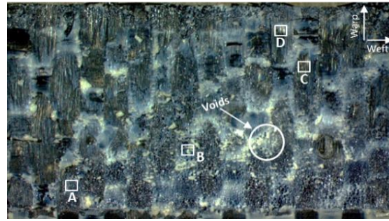
Figure 5.16. Fracture surface of an ANN_F specimen tested at -50°C showing cohesive failure accompanied by extensive areas of voids (e.g. circled area). A-D represent the locations at which the SEM micrographs were captured.
