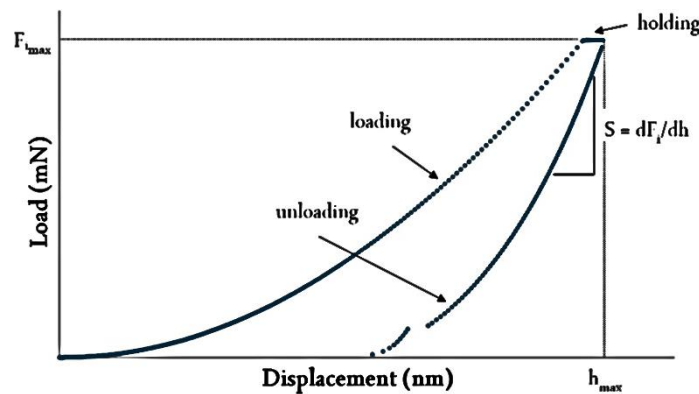
Figure 4.5. Schematic illustration of a typical load-displacement curve, adapted from [10].
