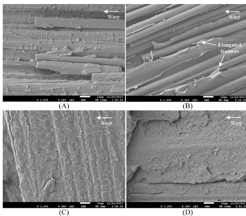
Figure 5.9. SEM micrographs of locations A-D of Figure 5.8 : (A) Broken and exposed fibres that still have matrix remnants on their surfaces. (B) Fibre distortion and extensive fibre/matrix debonding accompanied by considerable matrix drawing. (C) Smeared matrix indicating ductile failure. (D) Brittle failure as indicated by the limited plastic deformation. The arrow at the top right of each image indicates the warp direction.
