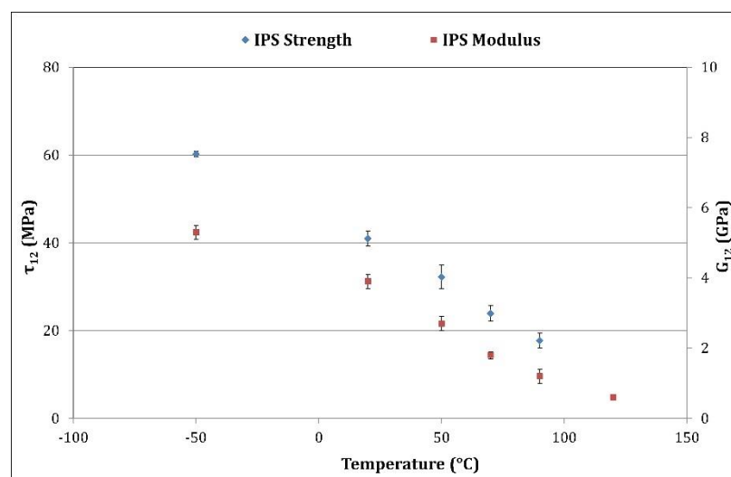
Figure 2.5. Effect of temperature on IPS properties of GF/PPS laminates. The scatter bars represent the standard deviation.
