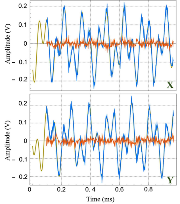
Fig. 5. Oscillation signal of the excited membrane mode, measured in the two quadratures at the output of the lock-in amplifier, in the period (0.1 \rightarrow 1.0)\text{ ms} after turning off the pump beam. As a consequence of the two heterodyne detections, i.e., the optical one with a local oscillator 12 kHz apart from the probe field, and the one performed by the lock-in amplifier with a local oscillator at 521.8 kHz, the oscillation at (525.8\text{ kHz} + f_m) splits into two sinusoidal signals at (8\text{ kHz} - f_m) and (16\text{ kHz} + f_m) . The experimental data (blue traces) are obtained from the average over 10 consecutive cycles, and are fitted with the expressions (4) and (5) (yellow lines). Red traces: residuals of the fits.
