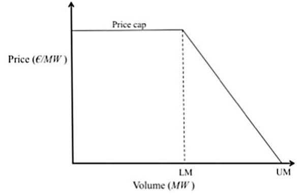
Fig. 5. Sloping demand curve used for clearing the CM with upper margin and lower margin from [166].
