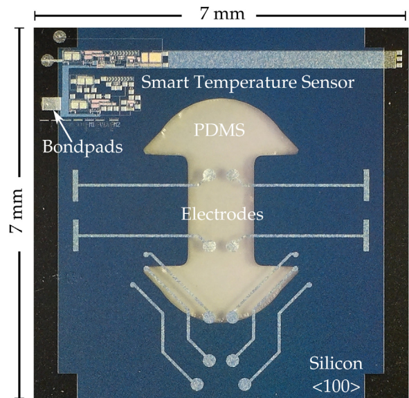
Fig. 4. Smart temperature sensor monolithically integrated on the Cytostretch chip.
