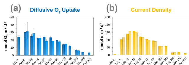
Figure 4. Time series of the (a) diffusive \text{O}_2 uptake in \text{mmol O}_2 \text{ m}^{-2} \text{ d}^{-1} and (b) current density as a consequence of long-distance electron transport ( e^- ) in \text{mmol e}^- \text{ m}^{-2} \text{ d}^{-1} in the sediment incubation.
