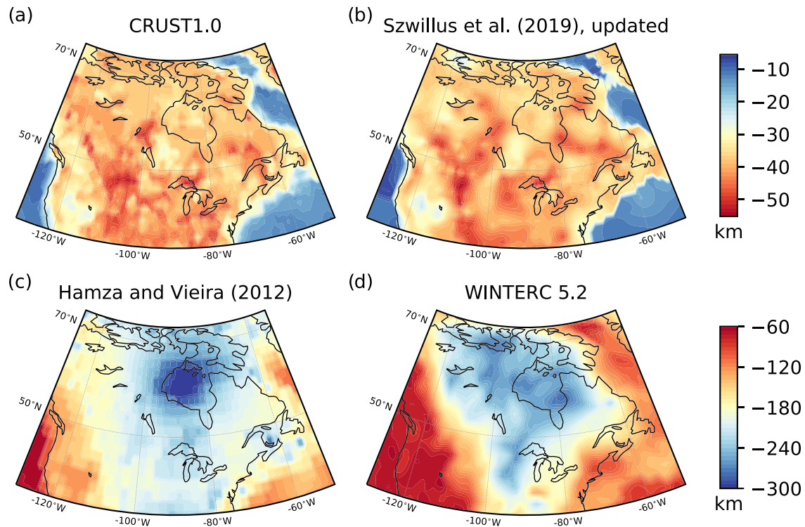
Figure 3. Moho depth of (a) CRUST1.0 (Laske et al., 2013) and (b) an augmented version of the Moho model compiled by Szwilius et al. (2019), as well as the LAB depth of (c) Hamza and Vieira (2012) and (d) WINTERC v5.2.
