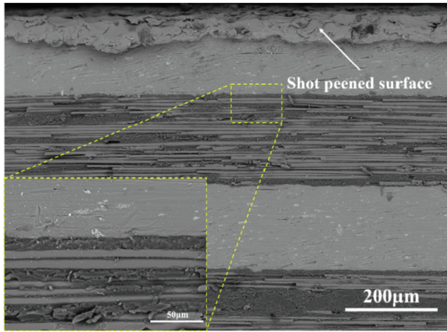
Fig. 7. The SEM morphology of shot peened FMLs.
