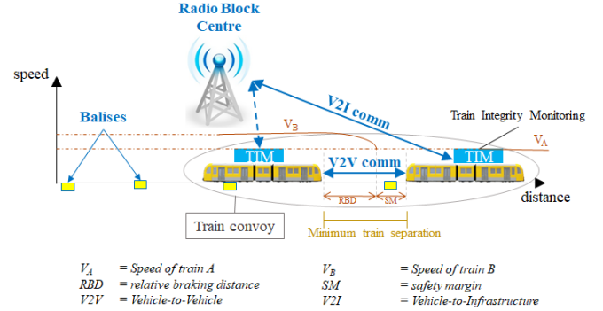
Figure 1. Schematic layout of Virtual Coupling train operations
