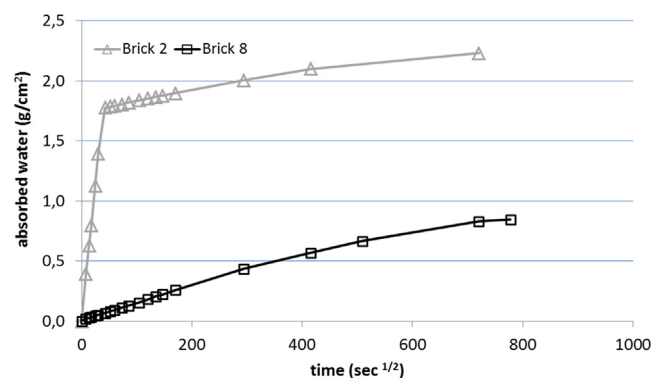
Fig. 4. Capillary water absorption curves of brick 2 and 8 (each curve is the average of measurements on 3 bricks).
