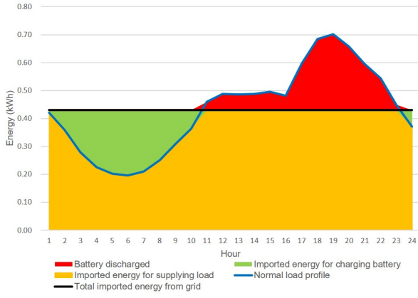
Fig. 1: An example of daily load flattening
