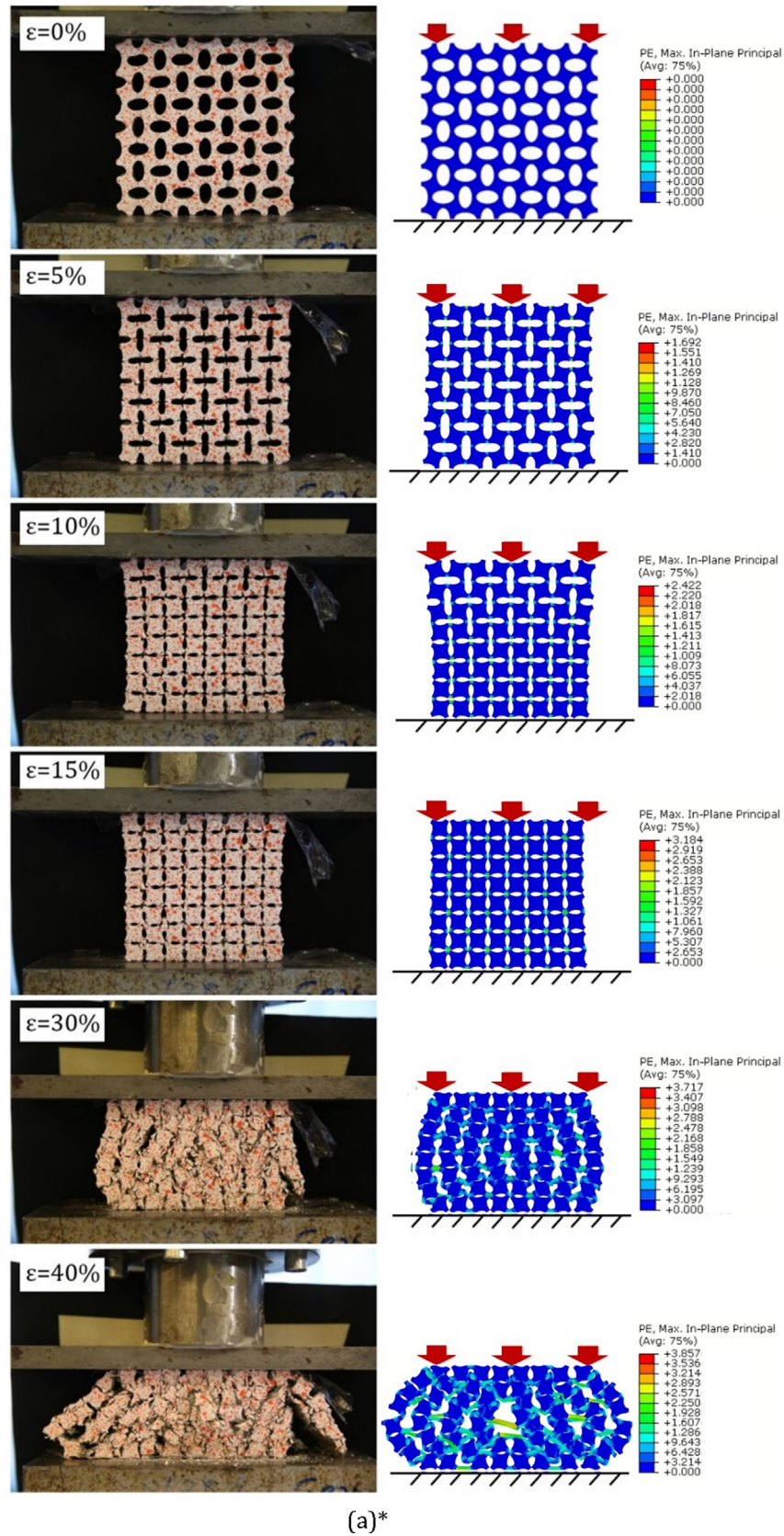
Fig. 9. Experiment and numerical simulated compression process of a) P25 and b) P50, *several experimental compression pictures of P25 are adopted from [27].
