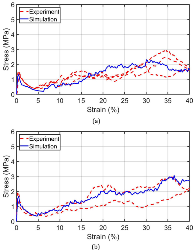
Fig. 18. Stress-strain curves of a) P25SG and b) P25DG obtained from experiment and simulation.
