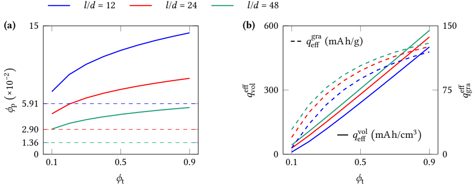
Fig. 2.15. Optimal conductive fiber volume fraction \phi_p (a) and the volumetric capacity q_{vol}^{eff} and gravimetric capacity q_{gra}^{eff} (b) versus total fiber volume fraction \phi_t at three different aspect ratios l/d . The dashed horizontal line in (a) denotes the percolation threshold \phi_{cr} . Material parameters for the active material ( \text{LiCoO}_2 ), conductive material, and solid polymer electrolyte can be found in Table 2.1.
