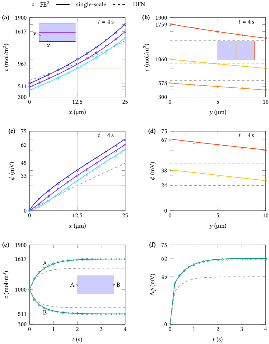
Fig. 4.6. Comparison between FE 2 calculation and single-scale simulations. Panels (a) and (c) show concentration c and potential \phi , respectively, along the x direction at y = 0, 5 , and 10 \mu\text{m} in the steady state ( t = 4 s); correspondingly, panels (b) and (d) show concentration c and potential \phi along the y direction at x = 0, 12.5 , and 25 \mu\text{m} . Here c and \phi refer to c_m and \phi_m for the FE 2 method, c_n and \phi_n for the DFN model (Table 4.1), and the intrinsic volume averages \langle c \rangle_\beta and \langle \phi \rangle_\beta for the single-scale simulations. Panel (e) shows the temporal evolution of the concentration at point A and B, which are located at the center of the leftmost ( x = 0 \mu\text{m} ) and rightmost ( x = 25 \mu\text{m} ) boundaries of the separator, respectively. Panel (f) shows the temporal evolution of the potential drop \Delta\phi from point B to A across the separator, i.e., the potential at point B, in view of a null potential fixed at the leftmost boundary.
