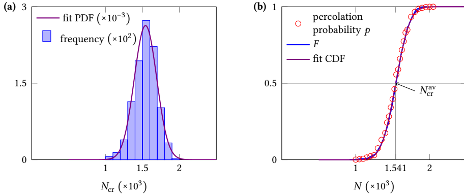
Fig. 2.6. Comparison of results between method A and B. Subfigure (a) shows histogram and fit (to normal distribution) probability density function of the 1000 critical fiber numbers N_{cr} from method B. Subfigure (b) shows the percolation probability at different conductive fiber numbers N from method A, the empirical cumulative probability F(N) by Eq. (2.19), and the fit cumulative distribution function of the 1000 critical fiber numbers N_{cr} from method B.
