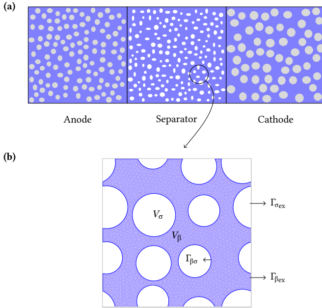
Fig. 4.1. Two-dimensional schematics of the problem domains. (a) Schematic of a battery cell with porous anode, separator, and cathode. The porous electrode and separator domains are filled with the electrolyte occupying domain V_\beta . (b) Microscopic representative volume element (RVE) of battery separator, consisting of blue-shaded electrolyte domain V_\beta and gray-shaded ion-transport blocking phase domains V_\sigma . The blocking phases represent the separator membrane. The RVE boundary \Gamma_{\text{ex}} is divided into two parts, each associated with a phase, such that \Gamma_{\text{ex}} = \Gamma_{\beta\text{ex}} \cup \Gamma_{\sigma\text{ex}} with \Gamma_{\beta\text{ex}} \cap \Gamma_{\sigma\text{ex}} = \emptyset .
