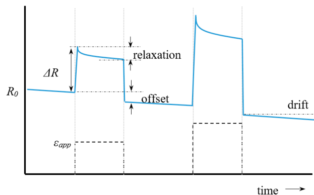
Figure 4. Schematic response of sensor after applied strain steps (black pulses).
