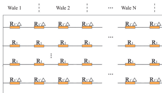
Figure 18. Simplified equivalent network model [68].
