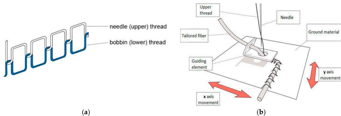
Figure 3. (a) Double lockstitch embroidery. The upper thread can be conductive; (b) Tailored fiber placement (TFP) embroidery; useful for fixating of functional fibers [34].
