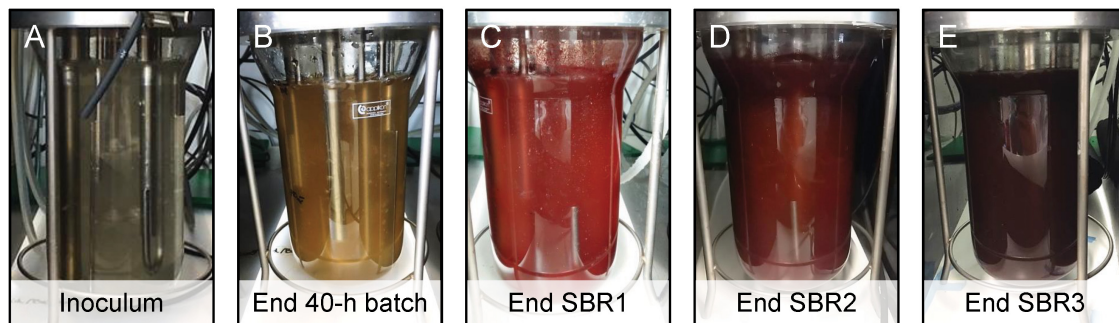
FIGURE 1 | Anaerobic stirred-tank photobioreactor operated in sequencing batch mode to enrich for and aggregate PNSB. (A) The reactor was inoculated at 0.1 \text{ gVSS L}^{-1} with BNR activated sludge. (B) One initial batch of 40 h was used to activate the sludge and test the enrichment of PNSB, prior to switching to SBR operations over 5 months. (C) SBR1 was operated with 1 cycle \text{d}^{-1} , HRT of 48 h, reaction phase of 20.75 h, and OLR of 0.215 \text{ g COD d}^{-1} \text{ L}_r^{-1} . (D) SBR2 was operated with 3 cycles \text{d}^{-1} , HRT of 16 h, reaction phase of 4.75 h, and OLR of 0.645 \text{ g COD d}^{-1} \text{ L}_r^{-1} . (E) SBR3 was run like SBR2 but fed at a doubled OLR of 1.290 \text{ g COD d}^{-1} \text{ L}_r^{-1} . The SRT was let freely evolve in the SBRs, increasing from 1.5 d ( SBR1 ) to 7.2 d ( SBR2 ) to 10.6 d ( SBR3 ) along with PNSB aggregation and accumulation in the system from 0.1 ( SBR1 ) to 1.6 ( SBR2 ) to 3.0 ( SBR3 ) \text{g VSS L}^{-1} .
