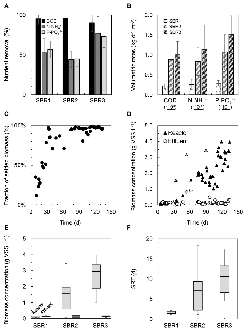
FIGURE 2 | Nutrient removal and biomass characteristics across SBR operations in the mixed-culture PNSB photobioreactor. (A) Increases in COD, ammonium, and orthophosphate nutrient removal percentages from SBR1 to SBR3. On average, 95% of the COD was removed during all operational states. N-NH 4 + and P-PO 4 3- reached 77 and 73% of removal from the synthetic influent. (B) Gradual increases in volumetric rates of C-N-P nutrient removals from SBR1 to SBR3. (C) Increase in the fraction of mixed-liquor biomass that settled in the bioreactor along SBR1 (days 3–30), SBR2 (days 30–100), and SBR3 (days 100–135) after inoculation with BNR activated sludge and a first batch of 40 h. (D) Accumulation of biomass in the photobioreactor from SBR1 to SBR2 and SBR3. The gray triangles relate to cleanings and resuspensions of the wall biofilm in the biosystem. They indicate the total amount of biomass that accumulated in the reactor. (E) Distributions of biomass concentrations in the reactor at the end of the reaction phase and in the effluent after settling. The settling ability of the biomass increased steadily during SBR operations. The residual biomass concentration in suspension at the end of the settling phase in SBR3 was 10 times lower than the concentration in the mixed liquor during reaction time, displaying the well-settling property of the PNSB-enriched biomass. (F) The SRT was let freely evolve in the reactor, increasing from median values of 2 days (SBR1) to 7.5 days (SBR2) and 11 days (SBR3) along with biomass accumulation.
