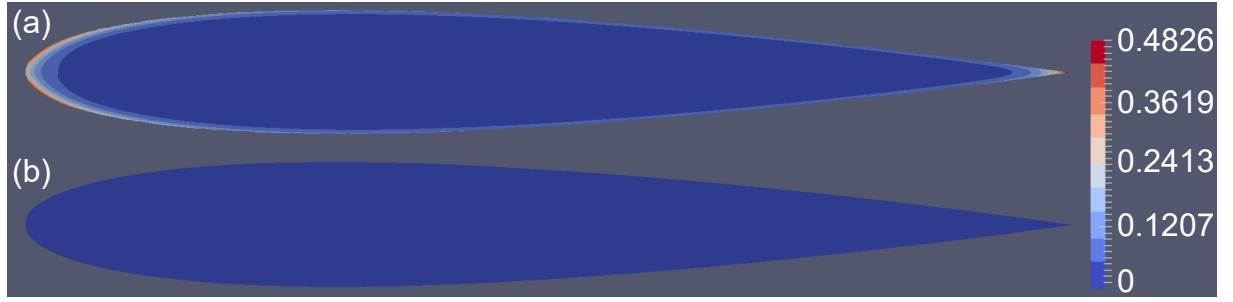
Figure 2: Flow past NACA0012 at Re=1000 modelled using (a) penalty forcing method and (b) domain decomposed method. The figure shows the magnitude of non-dimensionalised velocity inside the solid domain.
