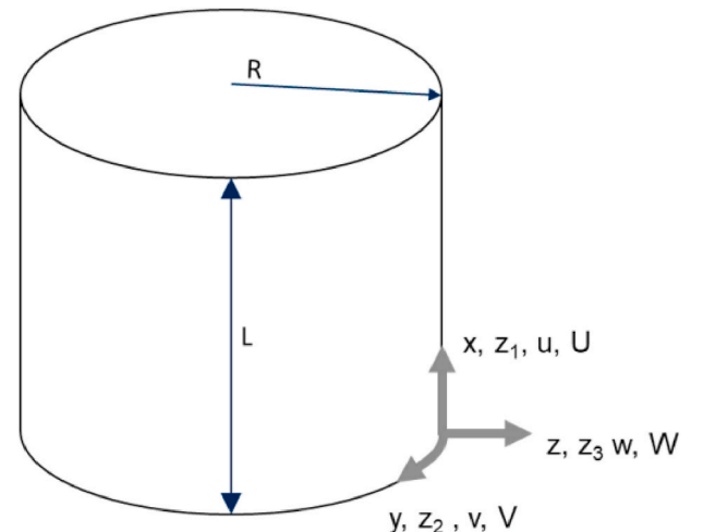
Fig. 2. Cylindrical shell geometry and coordinate system.
