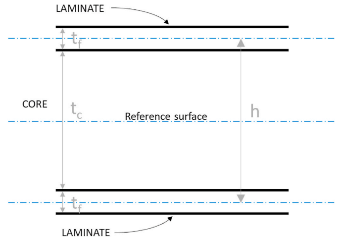
Fig. 1. Shell section.
