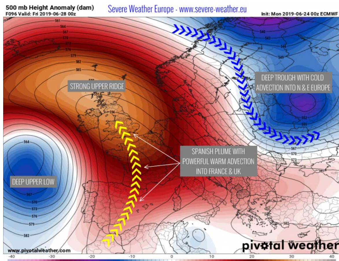
Figure 3 Heatwave Isobaric Chart for Europe 24-06-2019: (Pivotal Weather)
