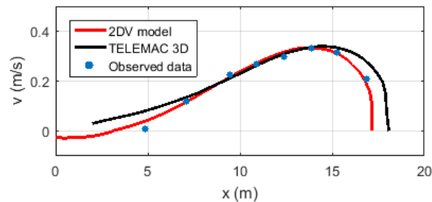
Figure 34. Longshore velocity at z = -2h/3 .
