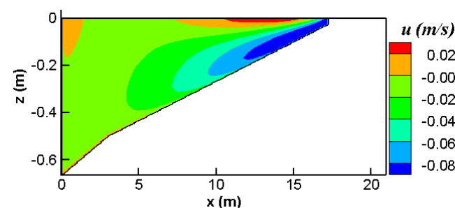
Figure 30. Distribution of cross-shore velocity.
