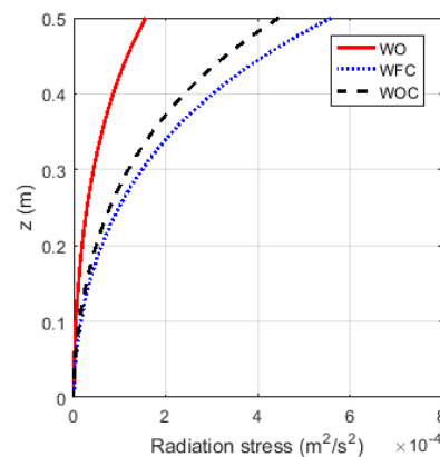
Figure 10. Vertical distribution of the wave radiation stress component \widetilde{u\widetilde{w}}_{CS} .
