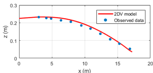
Figure 27. Distribution of significant wave height H_s .
