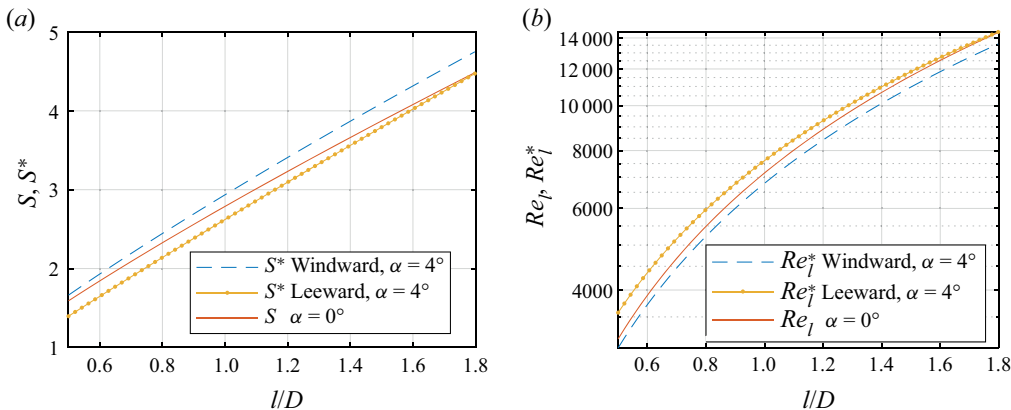
Figure 11. Correlation between the flow parameters from axial inflow ( S , Re_l at \alpha = 0^\circ ) and non-axial inflow ( S^* , Re_l^* at \alpha = 4^\circ ) along cone meridians (operating condition I: S_b = 5 and Re_L = 1.5 \times 10^4 ).
