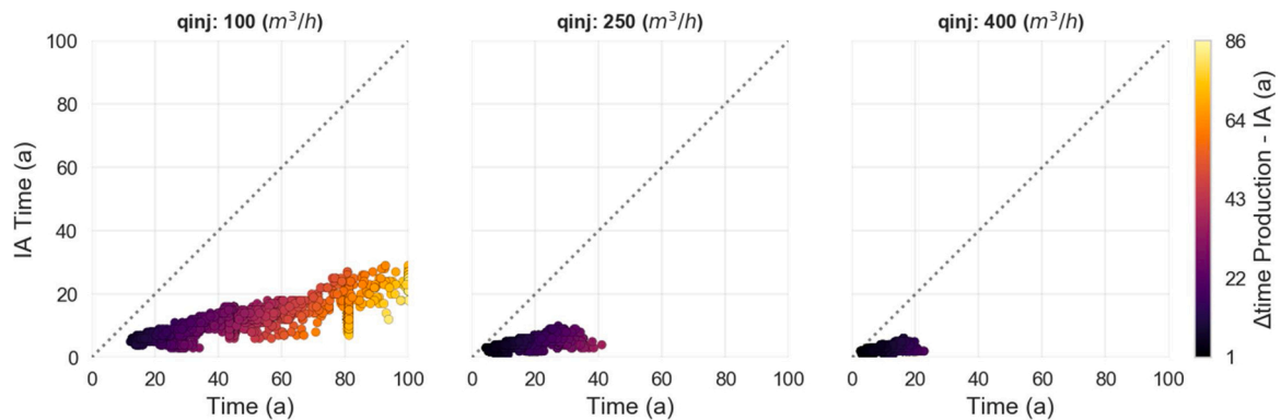
Fig. 23. Time of single developer production temperature drop of 1 °C (x-axis) to influence area (IA) time (y-axis) drop of 1 °C for the different flow rates considered. Data coloured according to the difference between system lifetime and influence area time, dotted line represents a 1:1 ratio. Full dataset of 5184 simulations is shown.
