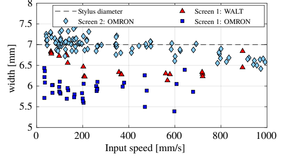
Fig. 7 Stylus width estimated from the vertical offset between the ‘top’ and ‘bottom’ regression lines.
