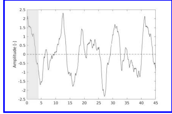
Fig. 3 Time trace of the multi-sine signal.
