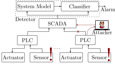
Figure 1: High level system and attacker model. The PLCs report sensor data about the anomalous process to the SCADA. The attacker can eavesdrop and manipulate a subset of the data provided to the SCADA. The reconstruction-based detector attempts to detect attacks based on a learned model of the system’s benign operations.
