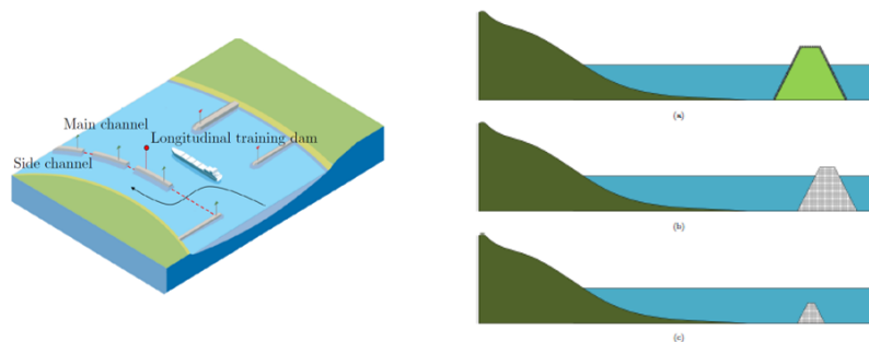
Figure 1 – Sketch of Longitudinal Training Walls (left) and cross sections of the longitudinal training structure (right a) and emerged and submerged sill (b and c) – [Jammers (2017)]
