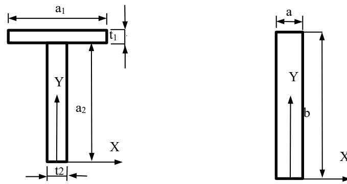
(a) T cross-section stiffener
