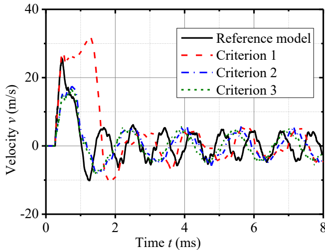
437 Fig. 16. Comparison of the velocity-time curves among the three criteria
