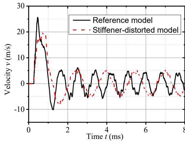
Fig. 20. Comparison of the velocity-time histories between the stiffeners distorted model and the reference model
