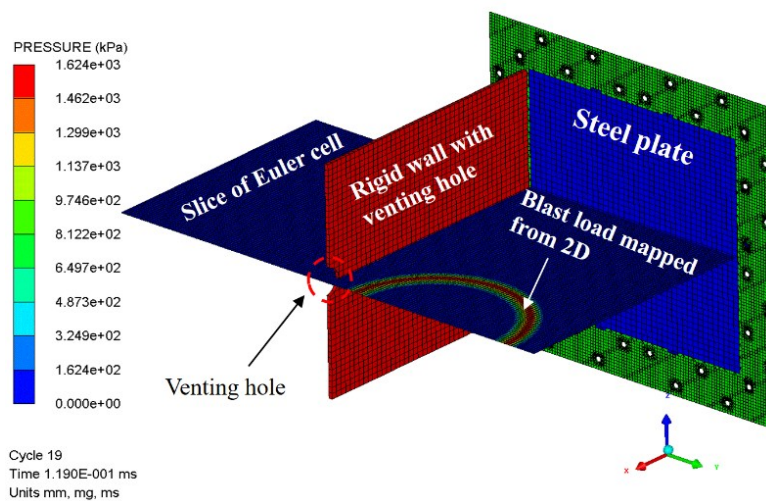
296 297 Fig. 10. The numerical model of fully Euler-Lagrange coupling calculation (half model)
