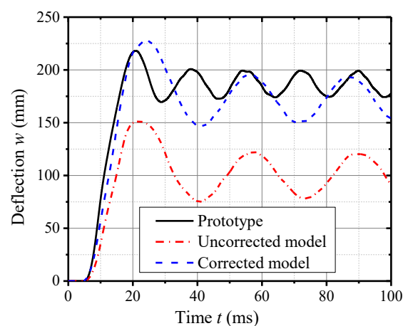
Fig. 21. Comparison of the deflection-time histories between prototype, uncorrected and corrected models
