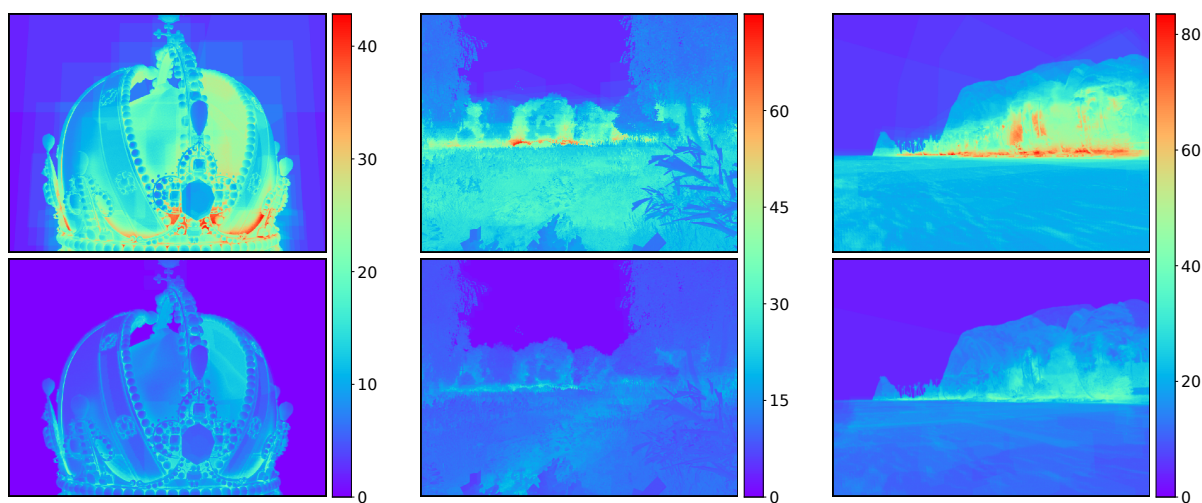
Figure 1: Our method reduces disk bandwidth by minimizing the number of batching points that need to be loaded. The images above show for each test scene (left to right: crown, landscape, island) the average number of batching points visited per sample in unidirectional path tracing. The top row shows regular batched ray traversal, the bottom row shows batched ray traversal with our method.
