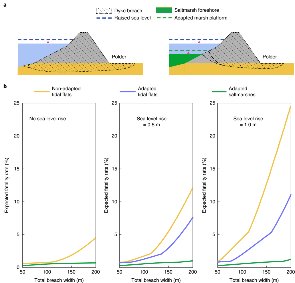
Fig. 5 | Relative advantage of saltmarsh foreshores over tidal flats in reducing flood impact under sea level rise. a, The rising sea level causes higher water depth on the sea side of the dyke without saltmarsh foreshores, whereas it remains unchanged in the presence of a saltmarsh foreshore that can keep pace with the rising sea level. b, The calculated fatality rate after dyke failure for three different foreshore scenarios: non-adapted tidal flats, adapted tidal flats and adapted saltmarshes. We assumed no delayed breaching process and no reduced breach width due to wave attenuation by saltmarshes to allow conservative comparisons between saltmarsh foreshores and bare tidal flats.
