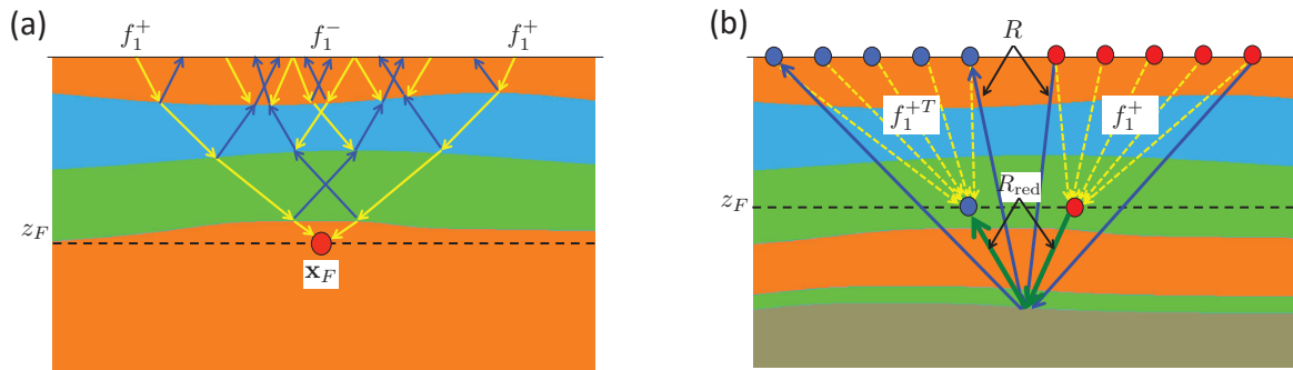
Figure 1 (a) Focusing function. (b) Redatuming by double focusing. The ‘rays’ represent primaries and multiples.
