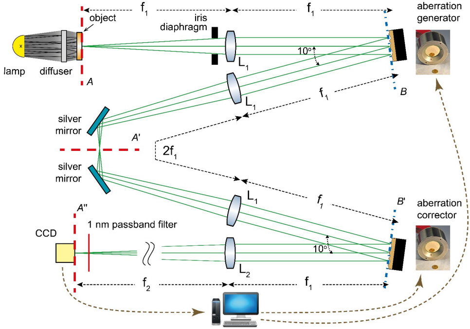
Figure 2.1: Sketch of the testbed. The plane of aberration generation (B) is imaged to the plane of aberration correction (B') with a 4-f telescope and a magnification of -1 . The letters A, A' and A'' indicate the image-forming conjugate planes. The magnification from plane A to plane A' is -1 , and from plane A' to plane A'' is -3 . The angles of incidence on the deformable mirrors are approximately 5^\circ . Due to the non-perpendicular incidence on the deformable mirrors, we place the two silver mirrors around plane A' to ensure the correct conjugation between the planes B and B'. Lenses focal lengths: f_1 = 250 mm, f_2 = 750 mm. An image captured with our testbed is shown in Fig. 2.2.
