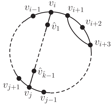
Figure 18. The induced subgraph R[V(C) \cup V(P)] .
