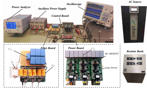
Fig. 6. Experimental setup.
