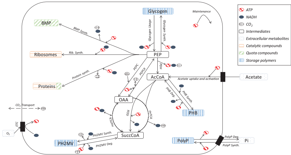
Figure 3.3: Simplified representation of the metabolic network used in this study. The complete reaction list and respective stoichiometries are shown in Table 3.1.
