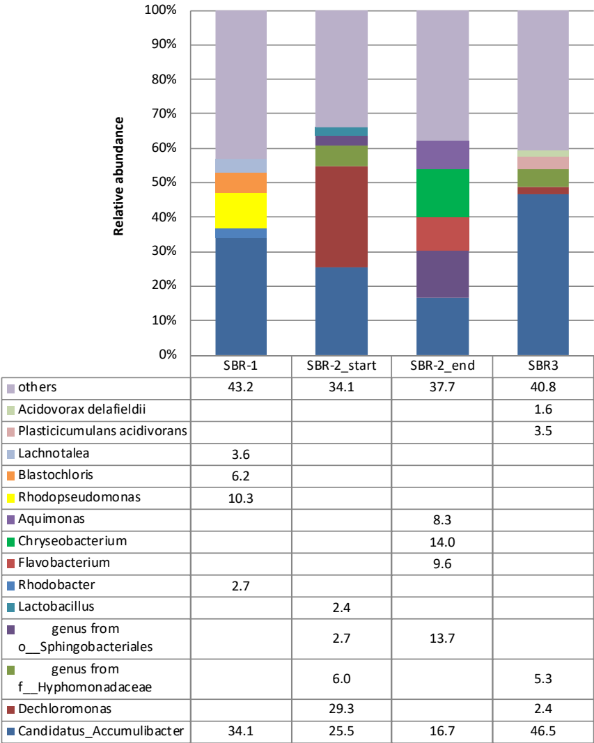
Figure 4.9: Taxonomic distribution of microbial community based on 16S rRNA gene copy numbers. The 16S rRNA gene amplicon libraries have been deposited under project PRJNA490689. SBR-3 was used in this study.
