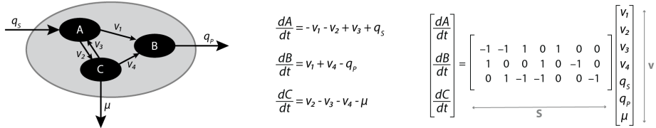
Figure 1.7: Simple model consisting in three metabolites (A, B, and C) with four reactions ( v_i ) and three exchange fluxes ( q_j ). The amount of A, B and C is described in time through mass balance equations. This system of ordinary differential equations can also be rewritten in matrix form. At steady state, the amounts of A, B and C do not change in time, thus S \cdot \mathbf{v} = 0 and the system gets reduced to an algebraic linear equations system. Adapted from (Kauffman, Prakash, and Edwards, 2003).
