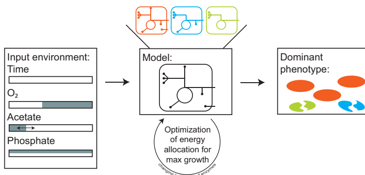
Figure 3.2: Overview of the approach used in this study. Cycle time and anaerobic/aerobic phases are fixed, while acetate uptake period and external phosphate availability are varied to create different environments.
