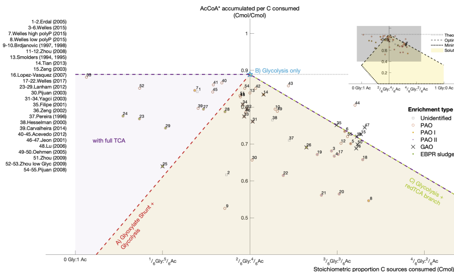
Figure 5.2: The amount of Ac-CoA* accumulated (PHB and PHV precursor) as a function of the proportion of glycogen to acetate consumed in the absence of an external electron acceptor. The yellow shaded area (below red and green dashed lines) corresponds to the possible stoichiometric combinations between acetate, glycogen and the different PHA precursors that are possible without a full TCA cycle. The purple area corresponds to the expansion of the possible combinations by assuming an active TCA cycle. Experimental datasets normalized to respect carbon and energy conservation principles (see Chapter 2 ). Adapted from Figure 2.22.
