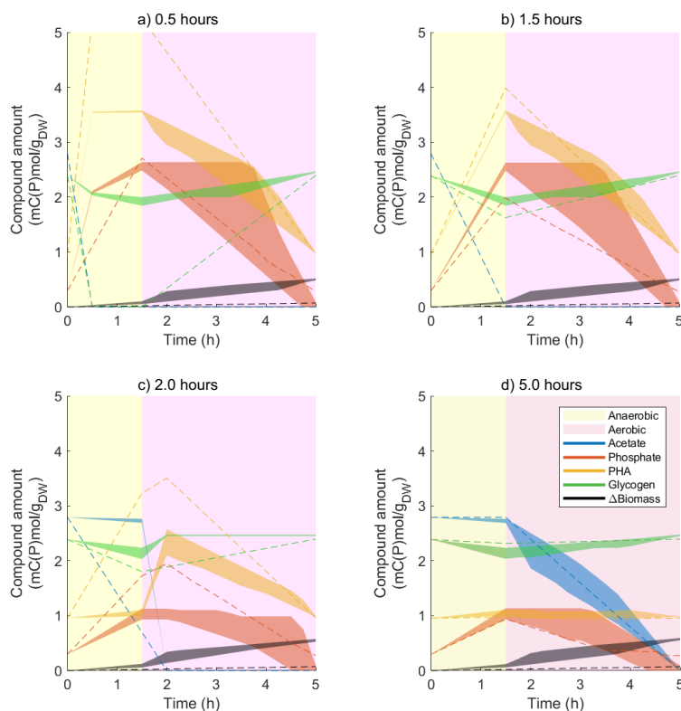
Figure 3.8: Simulated amounts of extracellular acetate and phosphate, intracellular polymers (PHA, glycogen) and lean biomass for the sensitivity analysis of the turnover rates ( k_{\text{cat}} ). Individual values of the different k_{\text{cat}} were changed by a factor of 0.1 and 10. Shaded areas represent the grouped output of all the simulations, except for the decrease of k_{\text{cat}} for BMP synthesis, which is represented by the dashed line. Amounts are normalized to the initial biomass amount. The phosphate profile is calculated from the polyphosphate dynamics and initial phosphate supplied in the medium (experimental). PHA is calculated from PHB and PH2MV. Scenarios: a) acetate uptake set to last only 30 min (same as in Figure 3.4); b) 1.5h; c) 2h and d) 5h.
