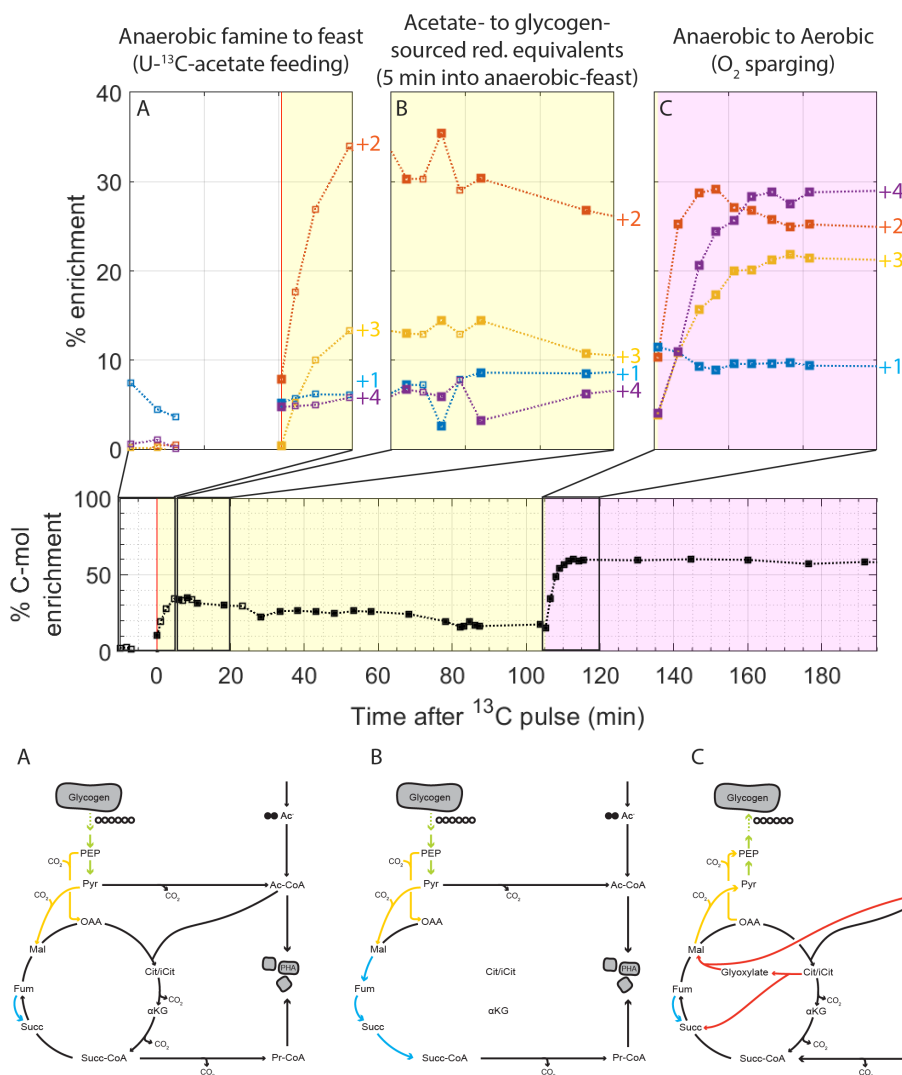
Figure 4.7: Comparison of the ^{13}\text{C} enrichment pattern of malate, i.e. relative proportion of mass isotopomers, stemming from different metabolic modes. A) acetate is added to the medium under anaerobic conditions and activated to acetyl-CoA that then flows through the TCA cycle, B) change in the ^{13}\text{C} enrichment trajectory likely because ^{13}\text{C} -acetyl-CoA is no longer being incorporated by citrate synthase and only ^{12}\text{C} -glycogen-derived precursors are entering the malate pool, C) oxygen becomes available and acetyl-CoA originates intracellularly from 60% ^{13}\text{C} -PHB and flows through both the TCA cycle and the glyoxylate shunt metabolic modes. Further analysis of different ^{13}\text{C} labelling patterns in malate depending on metabolic modes can be found later in Supplementary Table 4.2.
