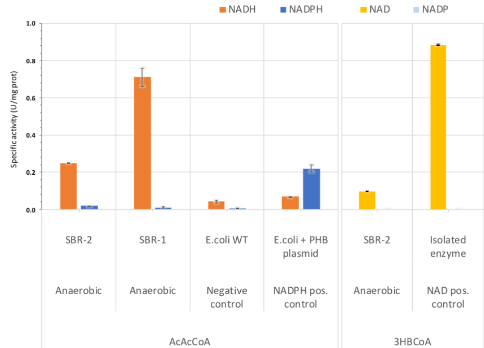
Figure 2.11: Accumulibacter acetoacetylCoA (AcAcCoA) reductase (step in PHA synthesis pathway) specific activity during the anaerobic phase. Note that in the assay with CFE from SBR-2 the used concentration of AcAcCoA was five times (5x) lower, hence the lower specific activity when compared to that of SBR-1. Specific activities during the aerobic phase are comparable and thus not shown here (see Table 2.5). Controls: (1) E. coli WT was used as negative control (still, a minor activity with NAD(H) is expected since this enzyme is also involved in fatty acids synthesis and is present in E. coli ), (2) E. coli with a PHB plasmid from R. eutropha was used as NADP(H)-positive control, and (3) Purified enzyme from Accumulibacter (overexpressed and purified in E. coli )
