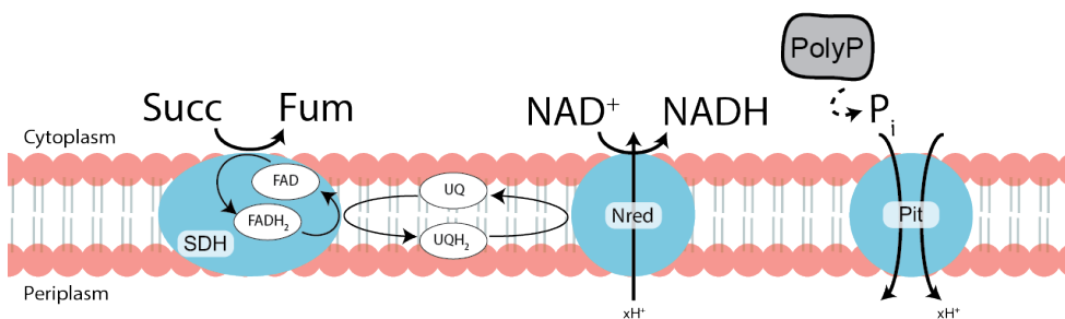
Figure 5.14: Proposed model for reversed electron transfer from succinate to \text{NAD}^+ at the cost of membrane potential, \Delta\Psi , generated by \text{P}_i -efflux.
