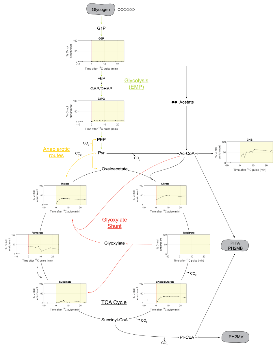
Figure 4.4: Measured ^{13}\text{C} enrichments during the anaerobic famine-to-feast transition. Bold squares are an average of both GC-MS/MS and LC-MS/MS methods. ATP and redox cofactors were omitted for simplicity. Isocitrate signal was below the detection limit throughout the whole anaerobic phase.
