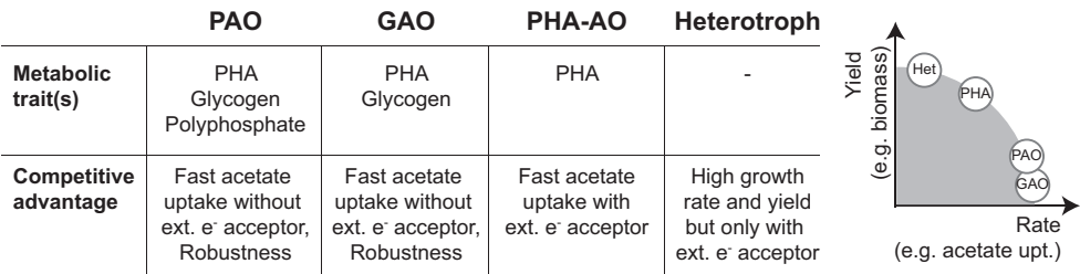
Figure 3.1: Main phenotypes found in activated sludge systems. Left: Metabolic traits and their respective competitive advantages. Right: Expected rate/yield trade-off curve. "Rate" can be seen as the competitive advantage of exclusive substrate uptake or substrate hoarding.
