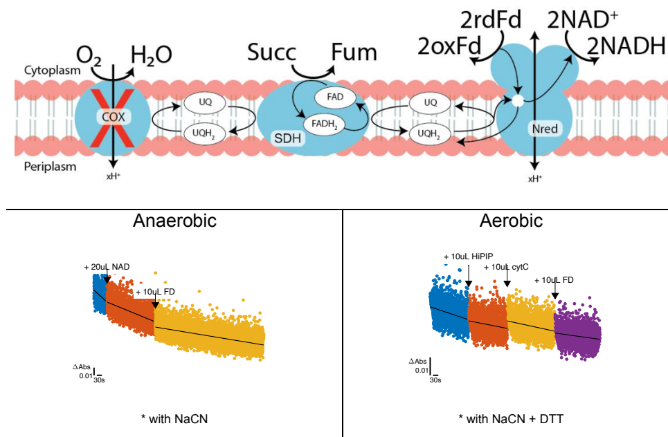
Figure 5.12: Reduction of \text{NAD}^+ by succinate and other electron donors (HiPIP, cytC, and Fd) in Accumulibacter membrane vesicles monitored at 340 nm. Cyanide (NaCN) was used to inhibit cytochrome oxidase activity (COX). Top reaction scheme – electrons are transferred from succinate to SDH, then to FAD, then the quinone pool and finally to \text{NAD}^+ . Left Nred activity of Accumulibacter harvested during the anaerobic phase. Reaction was triggered by the addition of ferredoxin (Fd). Right Nred activity of Accumulibacter harvested during the aerobic phase. Here the reaction was triggered by HiPIP, then cytC, and finally Fd. However, for all cases, the signal-to-noise ratio was too low to allow for accurate slope calculations and hence why activities could not be calculated and compared.
