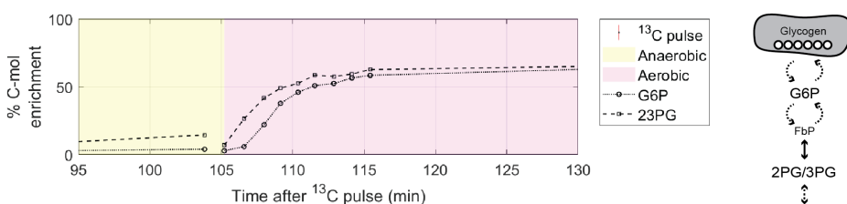
Figure 4.6: Comparison between G6P and 2-/3PG around the anaerobic-to-aerobic transition. Note the lag between 105 and 106 minutes for G6P while 2-/3PG are already getting ^{13}\text{C} -enriched.
