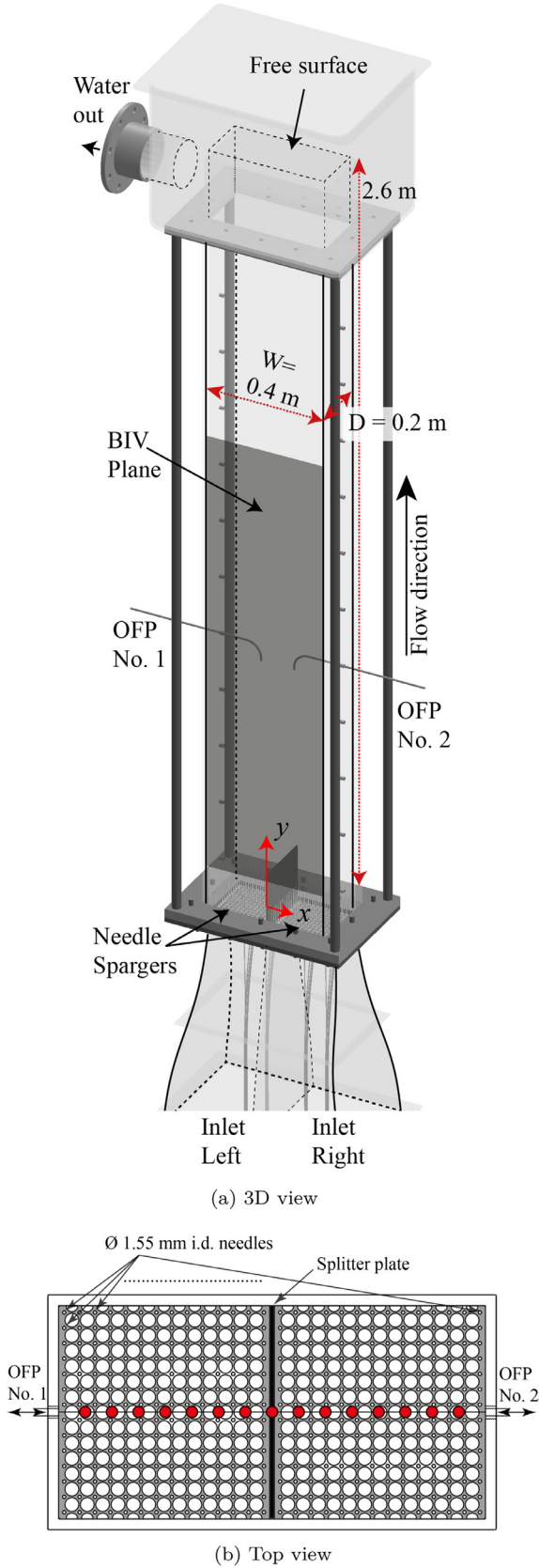
Fig. 1. Schematic drawing of the bubbly flow channel. Bubbles are formed on top of the needle spargers and air is separated from the water at the free surface. The Optical Fibre Probes (at a height of 40 and 80 cm above the needle spargers) are traversed in the x -direction along the center line of the column in steps of 2.5 cm, see red markers in (b). The needle sparger level, at y = 0 , is located 17 cm below the trailing edge of the splitter plate located. The experimental conditions are summarized in Table 1.
