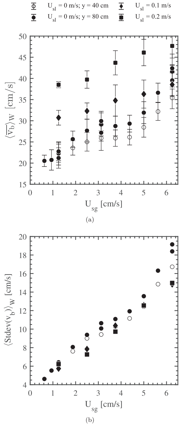
Fig. 11. (a) Time and horizontally averaged bubble velocities \langle \bar{v}_b \rangle and (b) standard deviations of \bar{v}_b as a function of the superficial gas velocity setting. The error bars denote the spread in (a) \bar{v}_b and (b) \text{Stdev}(v_b) with respect to the horizontal direction. The open markers show the results at y = 40 cm; the solid black markers show the data for y = 80 cm.
