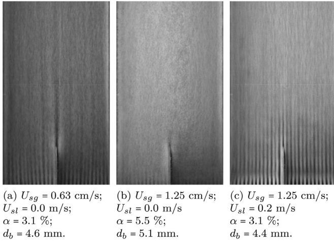
Fig. 6. Bubble streaks obtained by a 5 s simulated long exposure (image averaging technique). Corrected for lens distortion and contrast enhanced using a CLAHE technique. See Supplementary Material for the videos. The width of the images is 40 cm. Each inlet has an array of 14 \times 14 needles.
