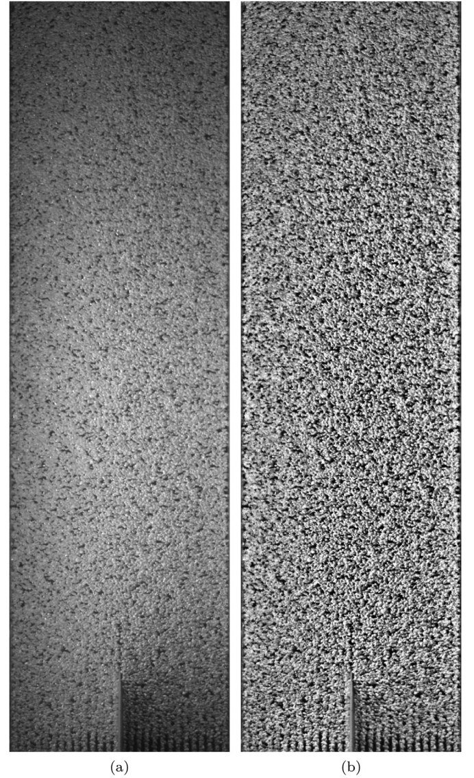
Fig. 2. Images of the bubble column. The field of view is 40 \times 140 cm ( W \times H ), starting \approx 2 cm above the needle sparger. (a) Raw image corrected for lens distortion. (b) Enhanced image using a contrast-limited adaptive histogram equalization (CLAHE) technique. U_{sg} = 1.67 cm/s. U_{sl} = 0.2 m/s.
