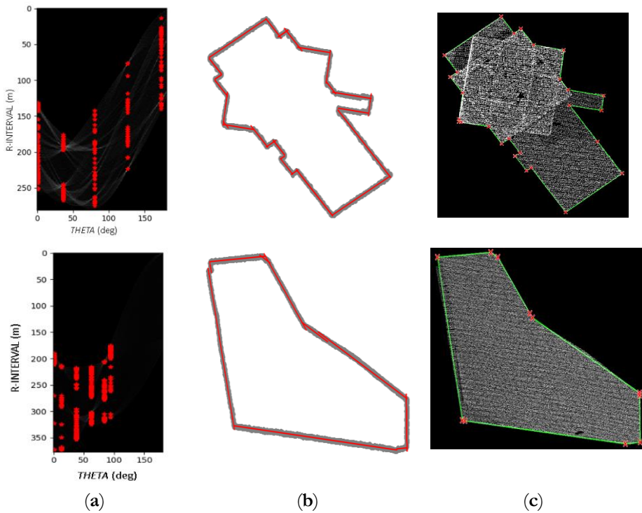
Figure 4.11 Extraction of buildings with multiple arbitrary directions. (a) Hotspots (red points) of multiple arbitrary directions; (b) Line detection; (c) Building outlines results.
