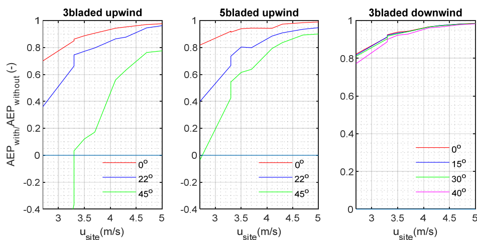
Figure 17. Ratio of Annual Energy Production with and without the standby losses plotted for increasing mean wind speed u_{\text{site}} (m/s) per different site and different yaw angles \theta ( ^\circ ).
