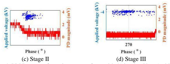
Fig. 4. PRPD pattern for staircase waveform with 41 level at V_p = 5.6 kV
