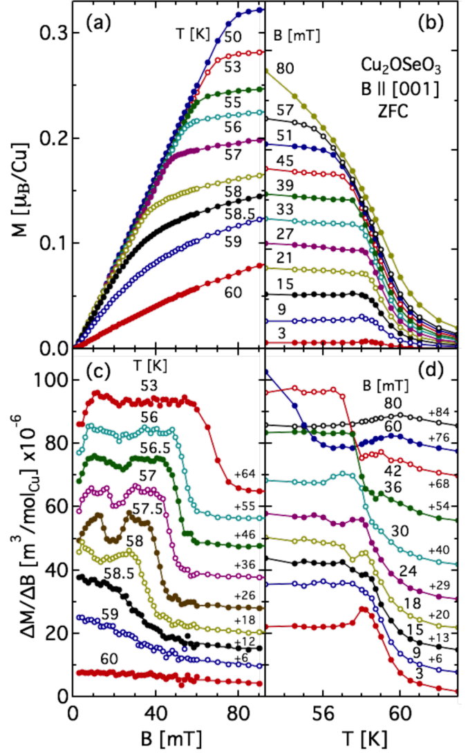
FIG. 2. ZFC magnetization of \text{Cu}_2\text{OSeO}_3 as a function of temperature and magnetic field. The same set of data has been plotted vs the magnetic field for selected temperatures (a) and vs the temperature for selected magnetic fields (b). The susceptibility \Delta M/\Delta B deduced by numerical differentiation of the M vs B curves is shown as a function of the magnetic field in (c) and of temperature in (d). For the sake of clarity the curves in (c) and (d) have been shifted vertically with respect to the baseline by the values indicated.
