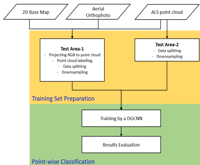
Figure 1. Methodological workflow used in this study to classify Airborne Laser Scanning (ALS) point clouds of two test areas using Dynamic Graph Convolutional Neural Network (DGCNN) architecture.
