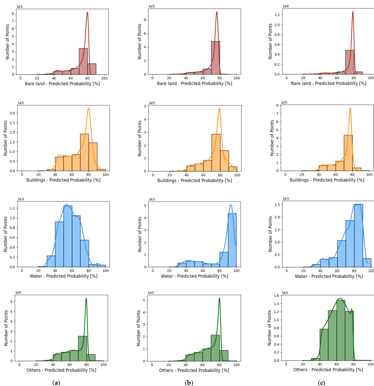
Figure 14. Per class probability distribution obtained by the network over test area with different block sizes (a–c). From top to bottom: class of bare land (1st row), buildings (2nd row), water (3rd row), and “others” (4th row).
