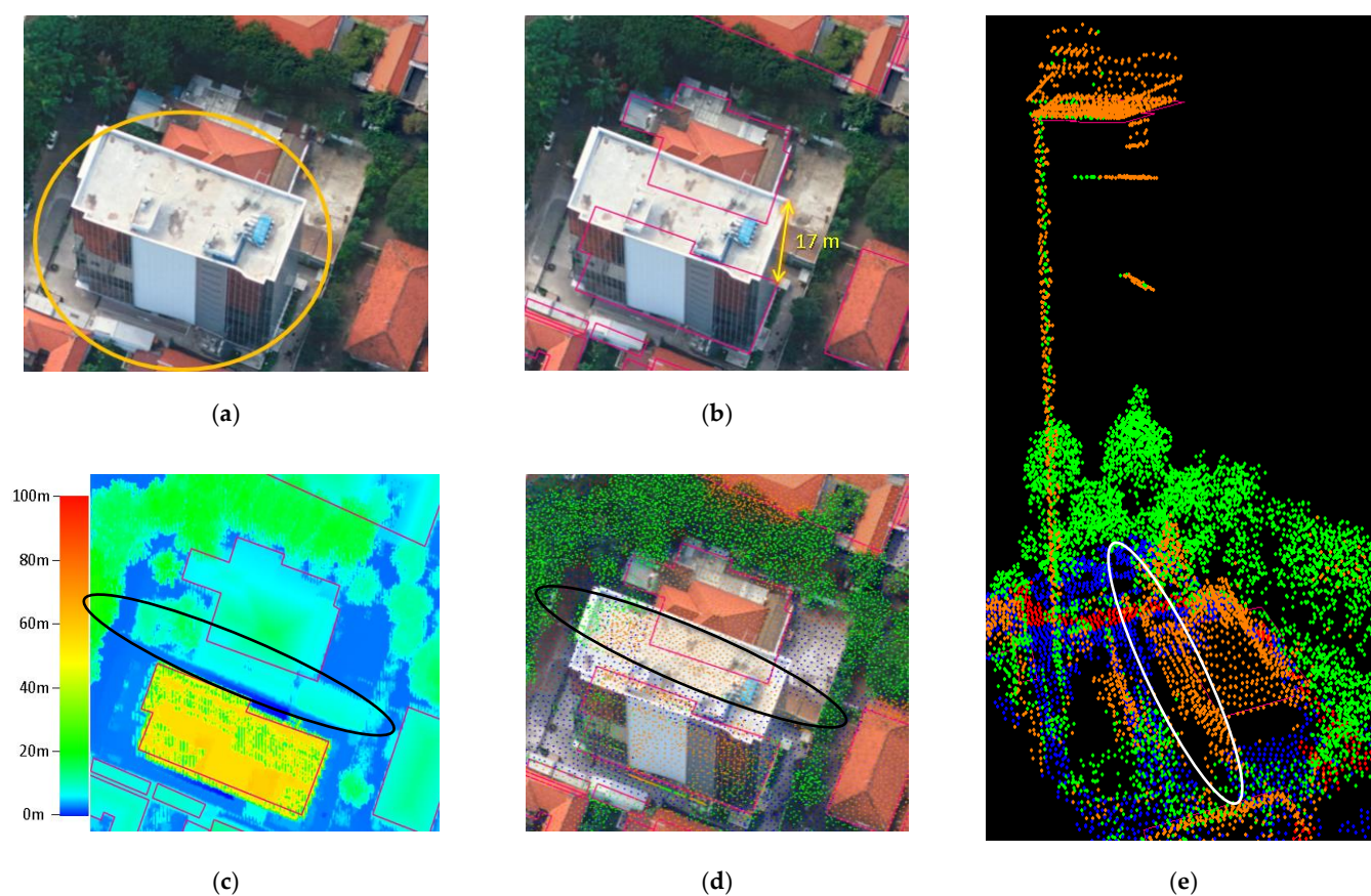
Figure 10. Relief displacement makes a high-rise building block an adjacent lower building and trees. (a) The leaning of a building (inside orange circle) on an orthophoto indicates relief displacement; (b) the building in the orthophoto has an offset of up to 17 m from the reference polygon (pink outlines); (c) the LiDAR DSM indicates a part of building that does not exist in the base map/reference (inside the black ellipse); (d) DGCNN can detect building points (orange) correctly, including the missing building part (inside the black ellipse); (e) 3D visualization of the classified building points including the missing building part (inside the white ellipse).
