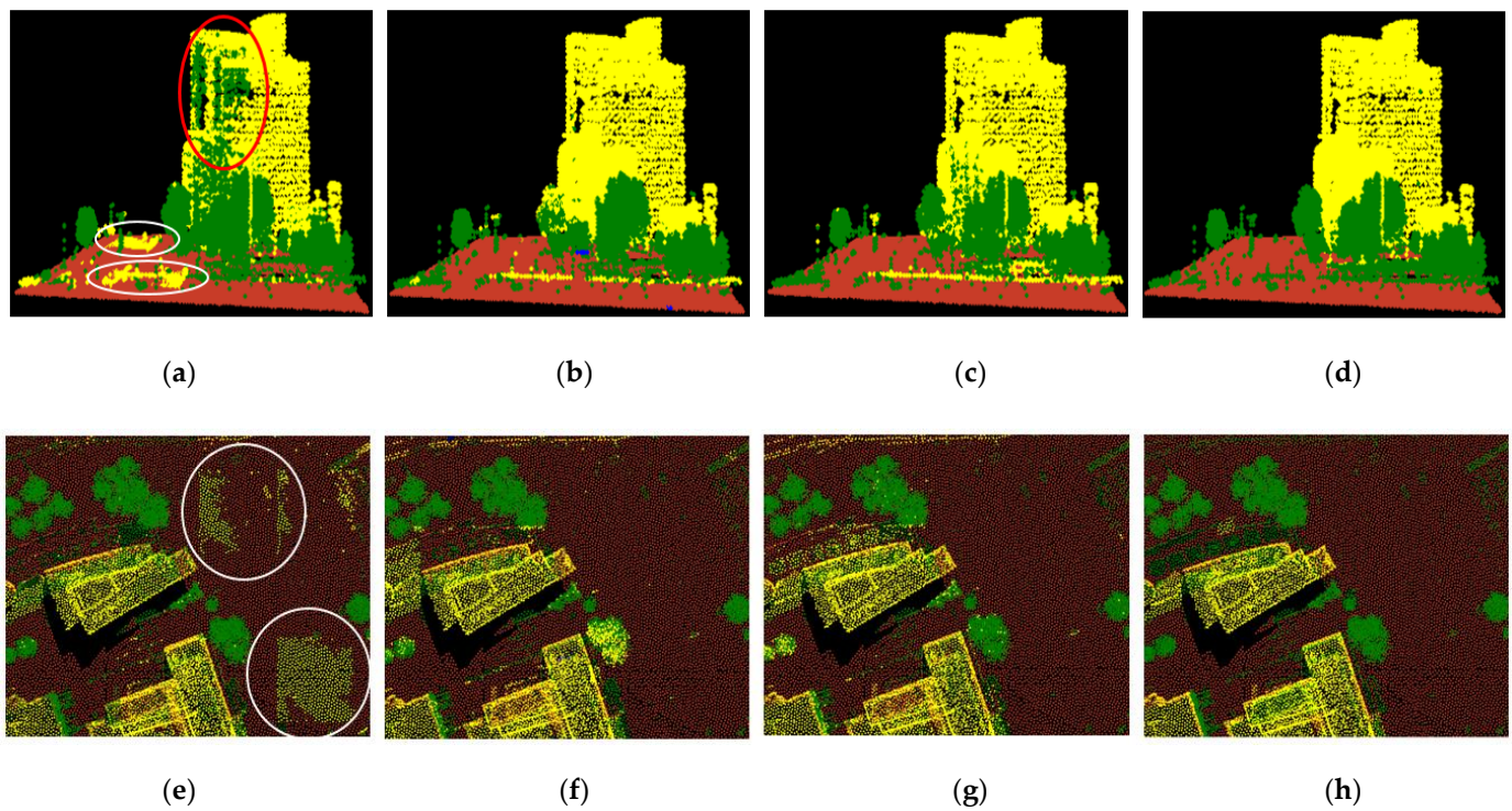
Figure 12. 3D visualization (a–d) and 2D visualization (e–h) of point cloud classification results of different block sizes and ground truths over a subset area of Area-2 (bare land in brown, buildings in yellow, water in blue and “others” in green).
