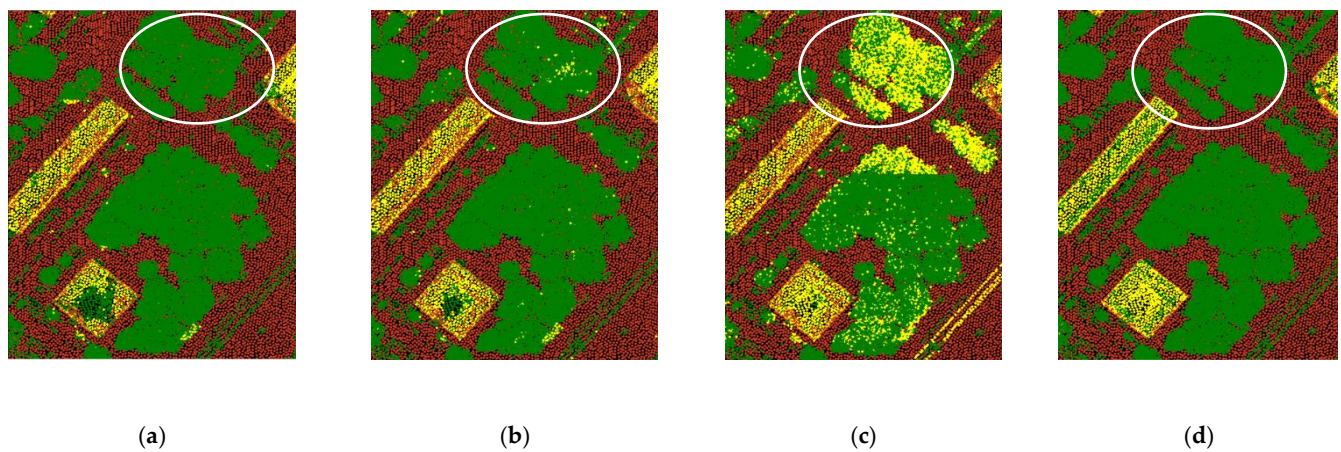
Figure 13. Comparison of point cloud classification results for different block sizes on a particular highly vegetated area show that bigger block sizes result in more misclassifications on trees (bare land in brown, buildings in yellow, water in blue and “others” (trees) in green). (a) Block size = 30 m, (b) block size = 50 m, (c) block size = 70 m, (d) ground truth.
