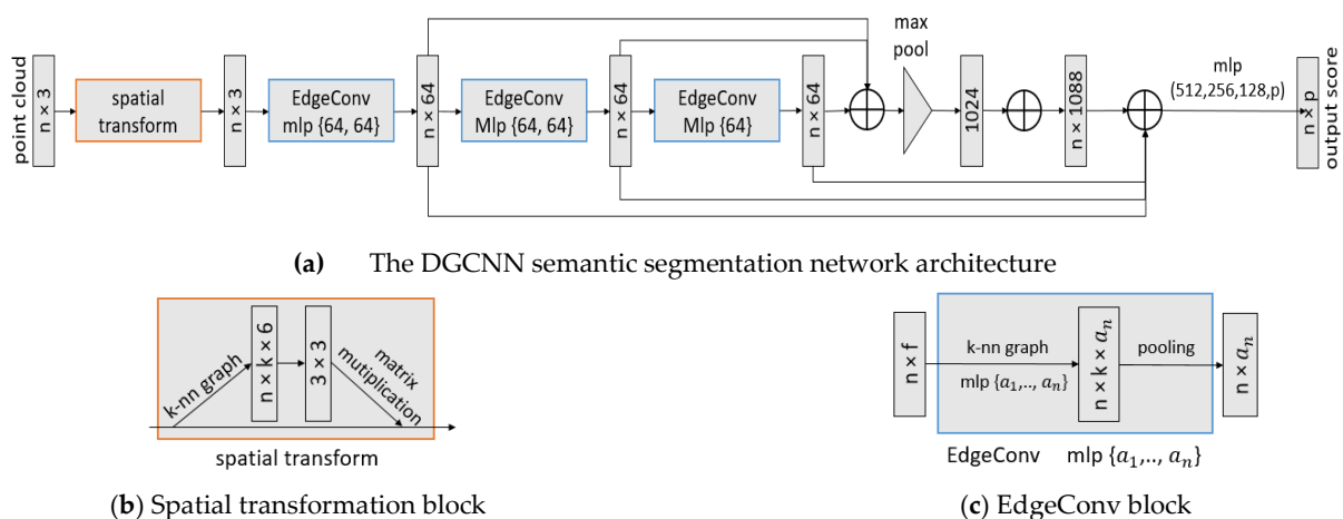
Figure 2. The DGCNN components for semantic segmentation architecture: (a) The network uses spatial transformation followed by three sequential EdgeConv layers and three fully connected layers. A max pooling operation is performed as a symmetric edge function to solve for the point clouds ordering problem—i.e., it makes the model permutation invariant while capturing global features. The fully connected layers will produce class prediction scores for each point. (b) A spatial transformation module is used to learn the rotation matrix of the points and increase spatial invariance of the input point clouds. (c) EdgeConv which acts as multilayer perceptron (MLP), is applied to learn local geometric features for each point. Source: Wang et al. (2018).
