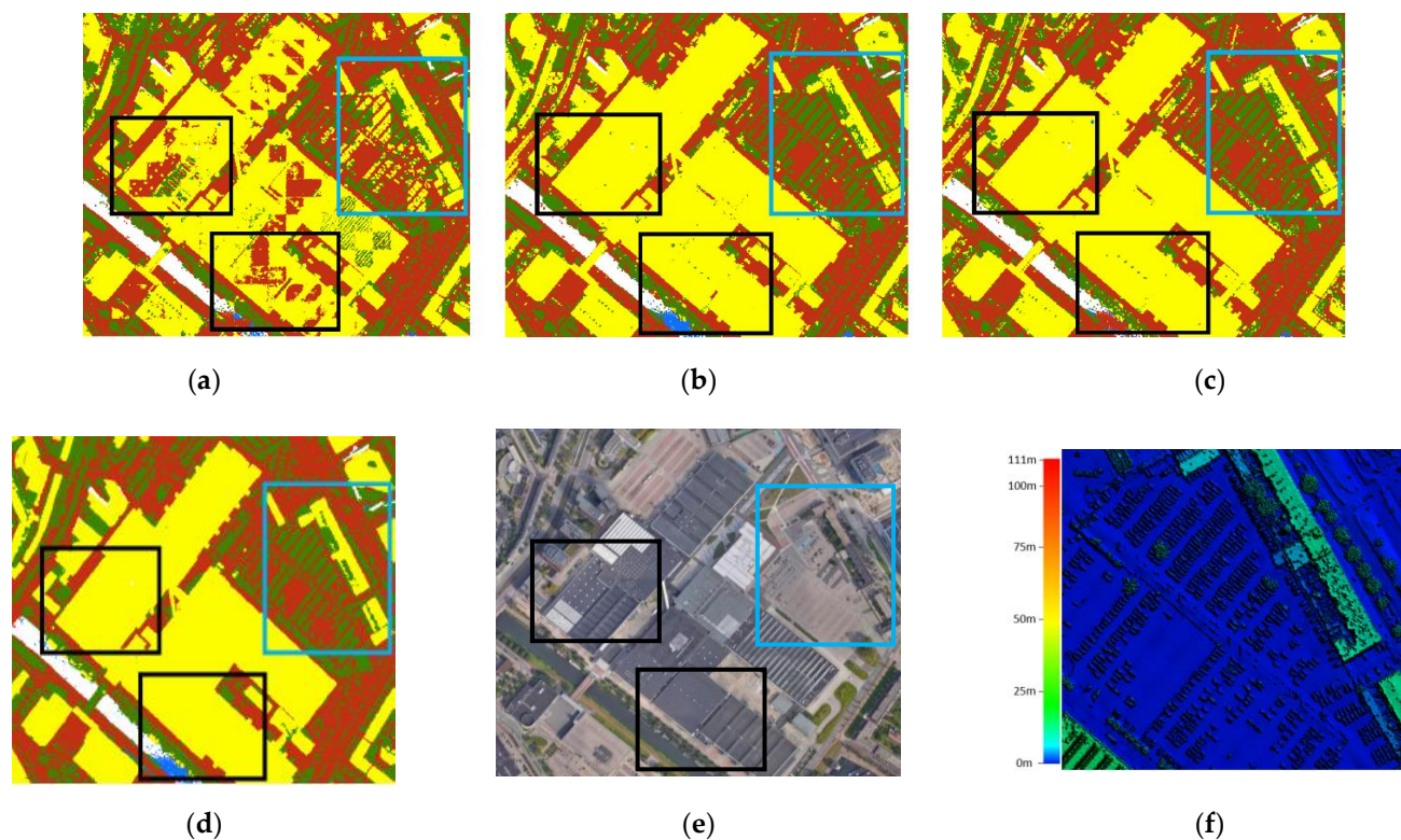
Figure 11. Visualization of point cloud classification results of a subtitle in Area-2 (bare land in brown, buildings in yellow, water in blue, and “others” in green) in comparison with the ground truth. (a) Block size = 30 m, (b) Block size = 50 m, (c) Block size = 70 m, (d) Ground truth, (e) Satellite image ©GoogleMap2020, (f) DSM of the blue box shows that cars are categorized as “others”.
