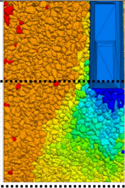
g. Vertical displacements of ballast particles at ballast shoulder (DEM)
