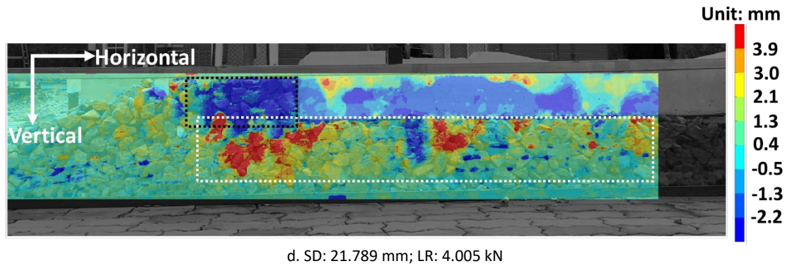
Figure 6 Vertical displacements of ballast particles at ballast bed cross section
