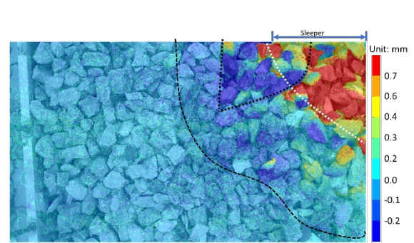
f. Horizontal displacements of ballast particles at ballast shoulder (PIV)
