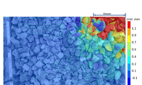
h. Vertical displacements of ballast particles at ballast shoulder (PIV)
