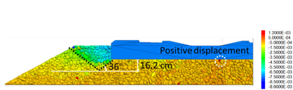
a. Horizontal displacements of ballast particles ballast bed cross section (DEM)
