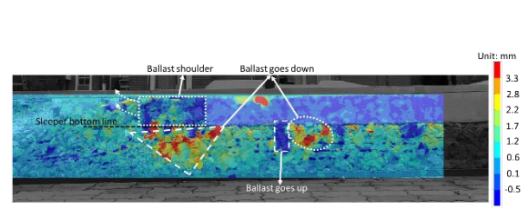
d. Vertical displacements of ballast particles at ballast bed cross section (PIV)
