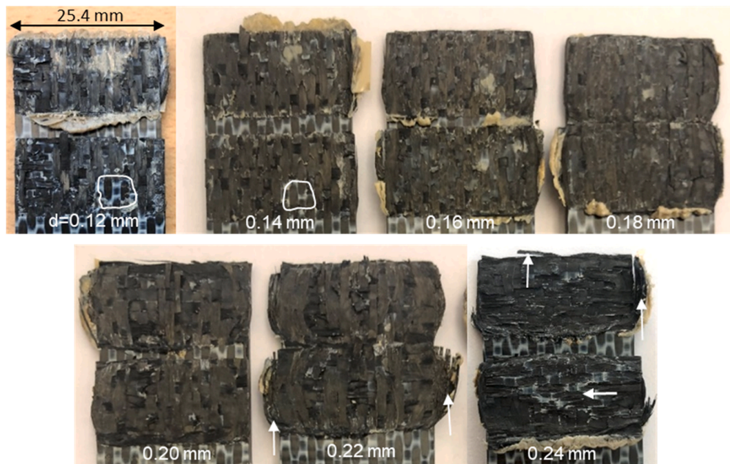
Fig. 10. Representative fracture surfaces of reference PEEK-PEEK samples welded at different displacement values. The displacement values of 0.14 mm, 0.18 mm and 0.22 mm correspond to the d_{low} , d_{opt} , and d_{high} , respectively. The size of the unwelded areas decreased with an increased target displacement. The unwelded areas are highlighted with white lines. The vertical arrows point at locations where significant fibre squeeze out was observed. The parallel arrow indicates failure between the first and second ply. (For interpretation of the references to color in this figure legend, the reader is referred to the web version of this article.)
