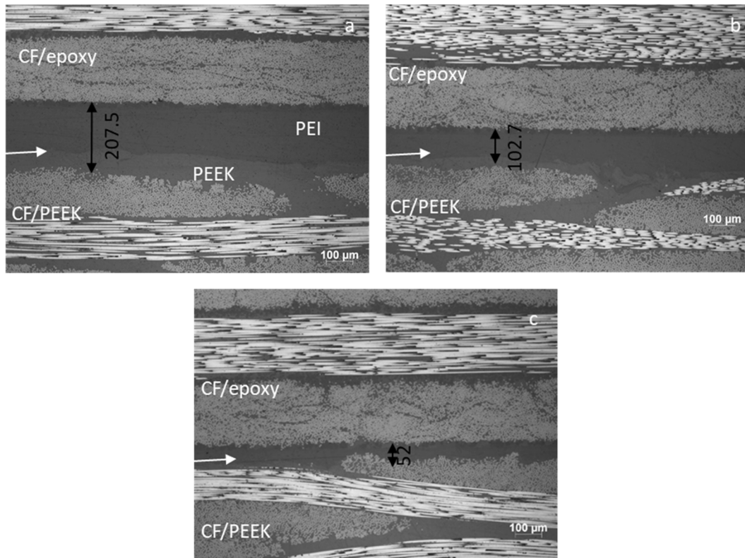
Fig. 3. Representative cross sections of epoxy-PEEK 250 samples welded at a displacement of a) 0.20 mm, b) 0.30 mm and c) 0.38 mm. The thickness of the weld line decreases with an increasing travel. White arrows indicate the weld line. The thickness measurements shown in the graphs are in \mu\text{m} .
