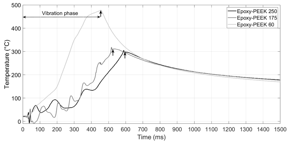
Fig. 16. Temperature evolution between the coupling layer and the CF/epoxy adherend for the considered epoxy-PEEK configurations. The samples were welded at d_{\text{high}} . Vertical arrows indicate the end of the vibration phase. Each sample contained one K-type thermocouple located at the middle of the overlap. The temperature was measured at 1000 Hz sampling rate.
