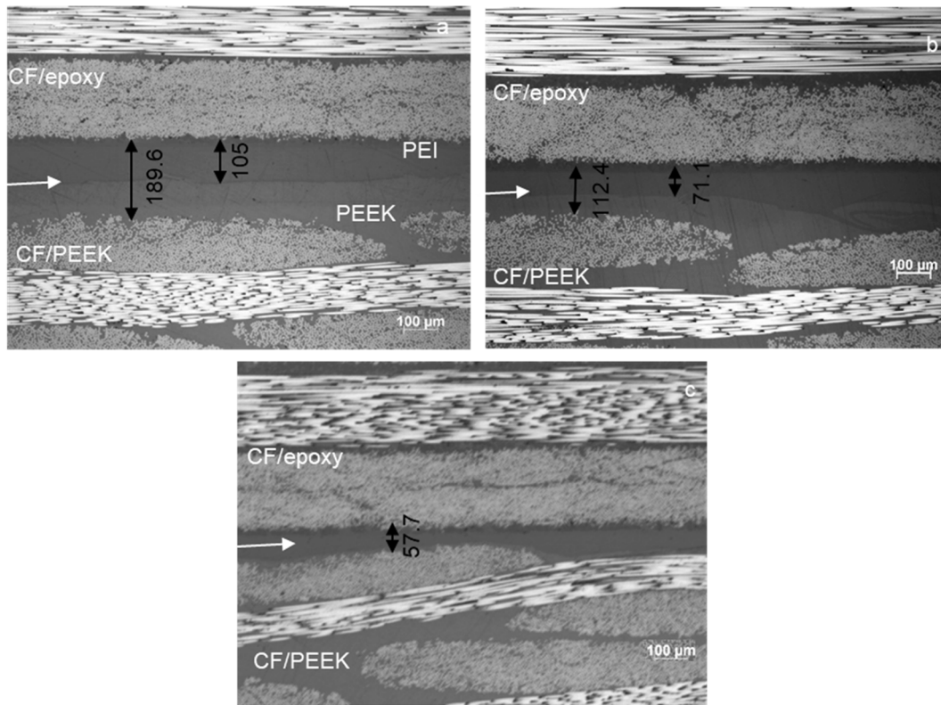
Fig. 15. Cross sections of epoxy-PEEK 175 samples welded at a displacement of a) 0.16 mm, b) 0.24 mm and c) 0.30 mm. White arrows indicate the weld line. The thickness measurements shown in the graphs are in \mu\text{m} .
