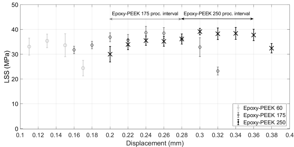
Fig. 12. Average lap shear strength of the epoxy-PEEK 250, epoxy-PEEK 175 and epoxy-PEEK 60 configurations versus the corresponding displacement.
