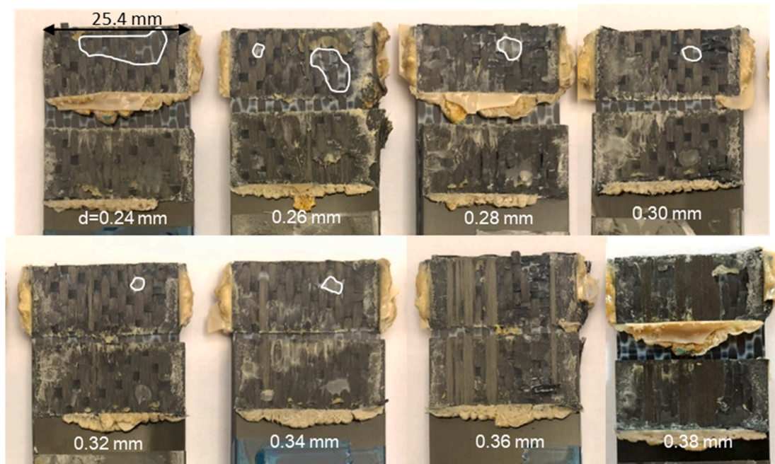
Fig. 8. Representative fracture surfaces of epoxy-PEEK 250 samples welded at different displacement values. The 0.28 mm, 0.30 mm and 0.36 mm values correspond to d_{low} , d_{opt} and d_{high} , respectively. The size of the unwelded areas (highlighted with white lines) decreased with an increasing target displacement. Welding at and above d_{high} resulted in failure in both adherends. (For interpretation of the references to color in this figure legend, the reader is referred to the web version of this article.)
