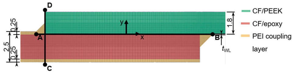
Fig. 2. 3D FE-model, central joint region for a single-lap design. The AB and CD paths correspond to the paths at which the peel and shear stresses were obtained. Dimensions are in [mm]. (For interpretation of the references to color in this figure legend, the reader is referred to the web version of this article.)
