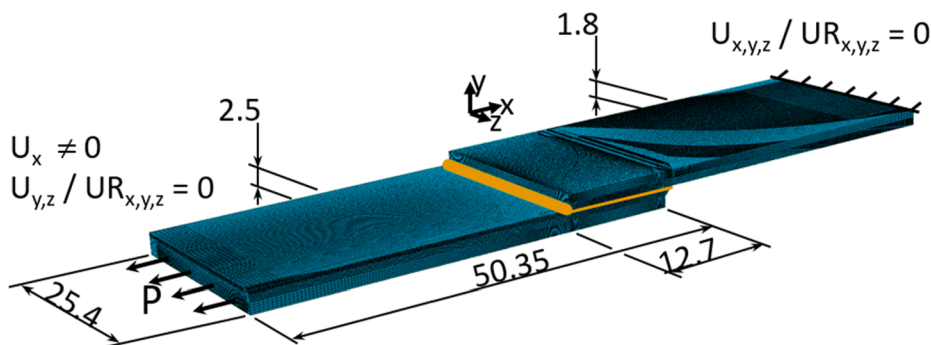
Fig. 1. 3D FE-model of the epoxy-PEEK 250 sample in a single-lap configuration, with boundary conditions. Dimensions are in [mm]. (For interpretation of the references to color in this figure legend, the reader is referred to the web version of this article.)
