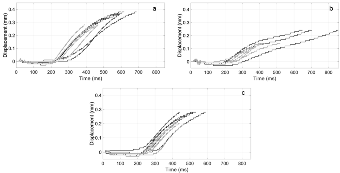
Fig. 14. Displacement of the sonotrode during the welding process in the a) epoxy-PEEK 250, b) reference PEEK-PEEK and c) epoxy-PEEK 175 configurations. Note: grey curves correspond to specimens welded up to d_{low} ; black curves correspond to specimens welded up to d_{high} (see Table 4).
