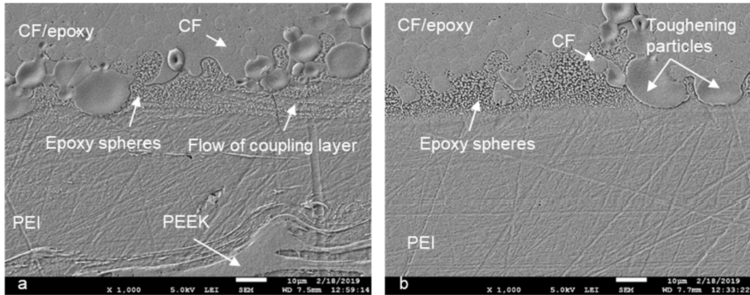
Fig. 4. Representative SEM cross-sectional micrographs of epoxy-PEEK 250 samples welded at a displacement of a) 0.38 mm and b) 0.30 mm. The epoxy-PEI interphase seems intact when samples are welded at d_{\text{opt}} whereas flow of the coupling layer close to the epoxy resin, leading to alteration of the original interphase morphology is observed when the samples are welded above d_{\text{high}} .
