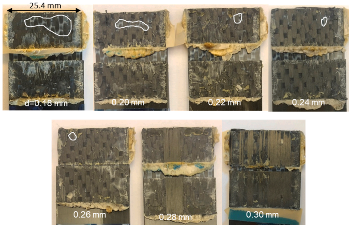
Fig. 13. Representative fracture surfaces of epoxy-PEEK 175 samples welded at different displacement values. The displacement values of 0.20 mm, 0.24 mm and 0.28 mm correspond to the d_{low} , d_{opt} and d_{high} , respectively. (For interpretation of the references to color in this figure legend, the reader is referred to the web version of this article.)
