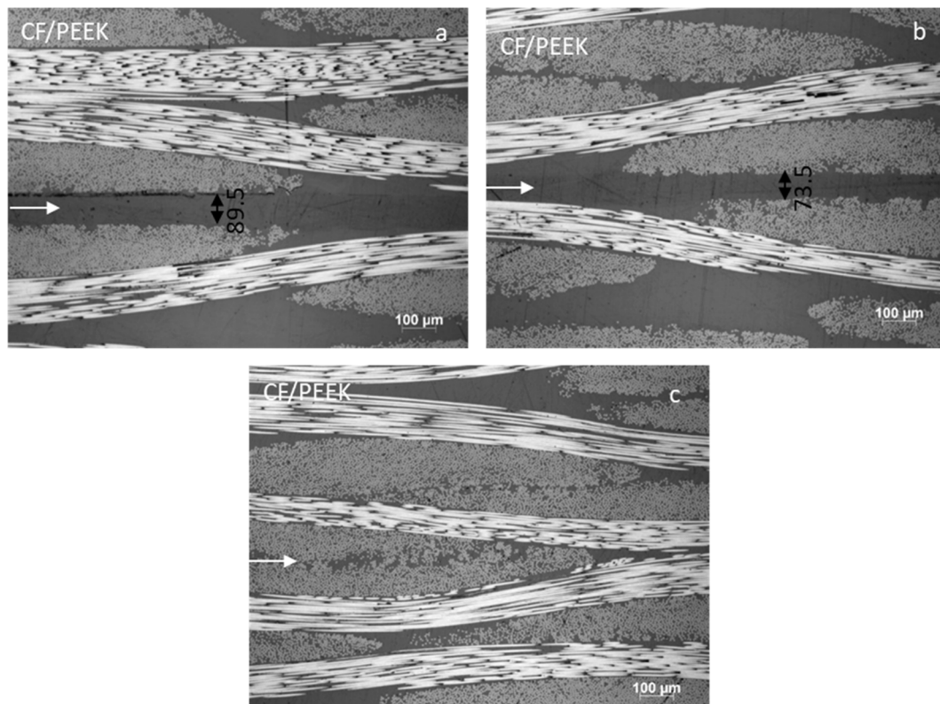
Fig. 5. Representative cross sections of reference PEEK-PEEK CF/PEEK samples welded at a displacement of a) 0.12 mm, b) 0.18 mm and c) 0.24 mm. The thickness of the weld line decreases with increasing displacement. White arrows indicate the weld line. The thickness measurements shown in the graphs are in \mu\text{m} .
