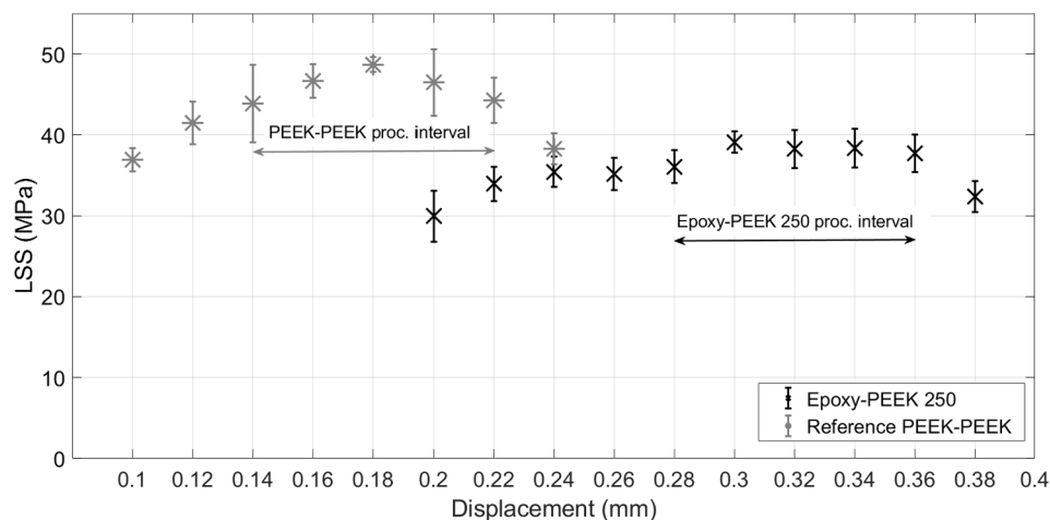
Fig. 7. Average lap shear strength of the epoxy-PEEK 250 and reference PEEK-PEEK configurations versus sonotrode displacement. The processing intervals were defined based on average LSS values higher than 90% of the maximum achieved LSS within the configuration.
