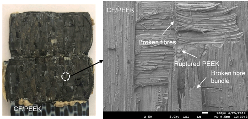
Fig. 11. Closer inspection of the fracture surfaces of a reference PEEK-PEEK sample welded at d_{opt} , showing failure in the CF/PEEK adherend, characterized by ruptured resin and broken fibres. The SEM image is representative of the whole overlap. (For interpretation of the references to color in this figure legend, the reader is referred to the web version of this article.)
