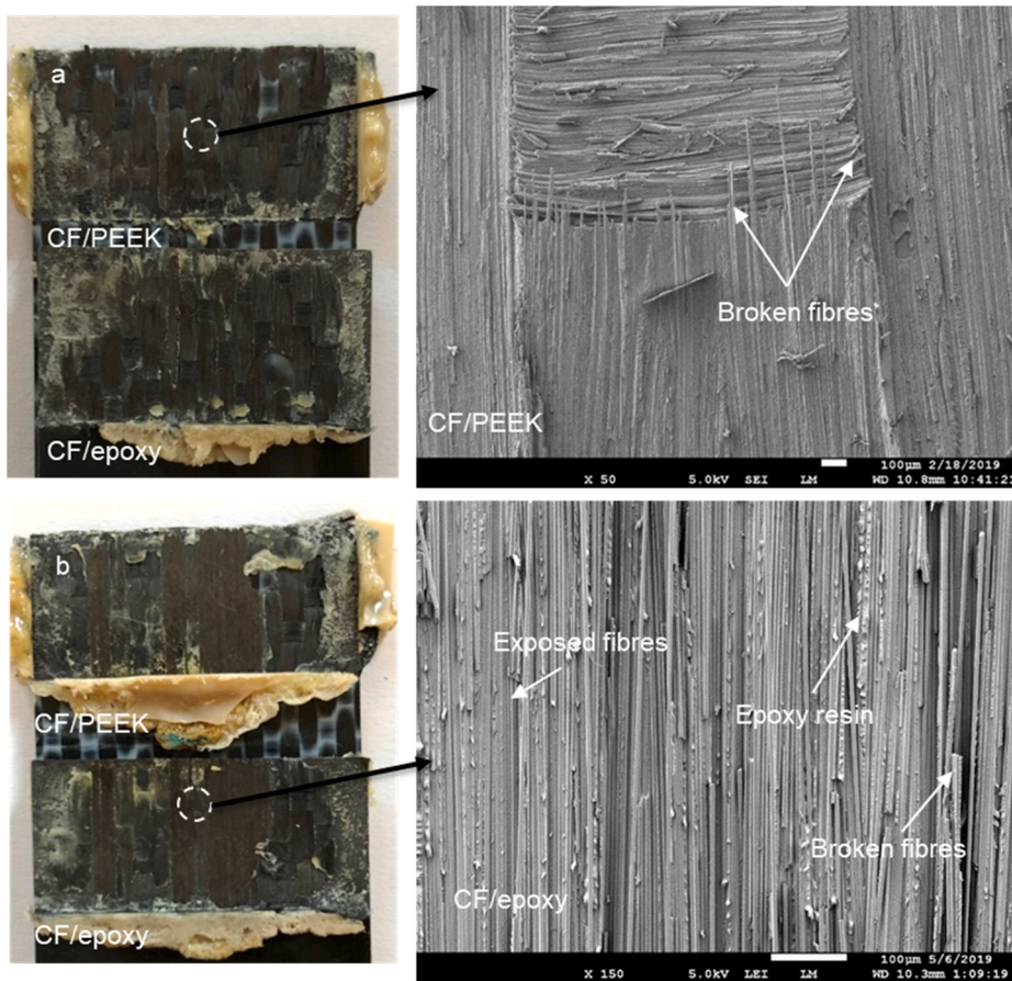
Fig. 9. Closer inspection of the fracture surfaces of epoxy-PEEK 250 joints welded at a) 0.30 mm, i.e., d_{opt} , showing failure in the CF/PEEK adherend, characterized by resin-rich fibre bundles, ruptured PEEK matrix, and broken fibres and b) at 0.38 mm, i.e. right above d_{high} , depicting failure in both adherends with failure in the CF/epoxy adherend characterized by mainly exposed fibres and broken fibres. The SEM images are representative of the whole area in which either type of failure occurred. (For interpretation of the references to color in this figure legend, the reader is referred to the web version of this article.)
