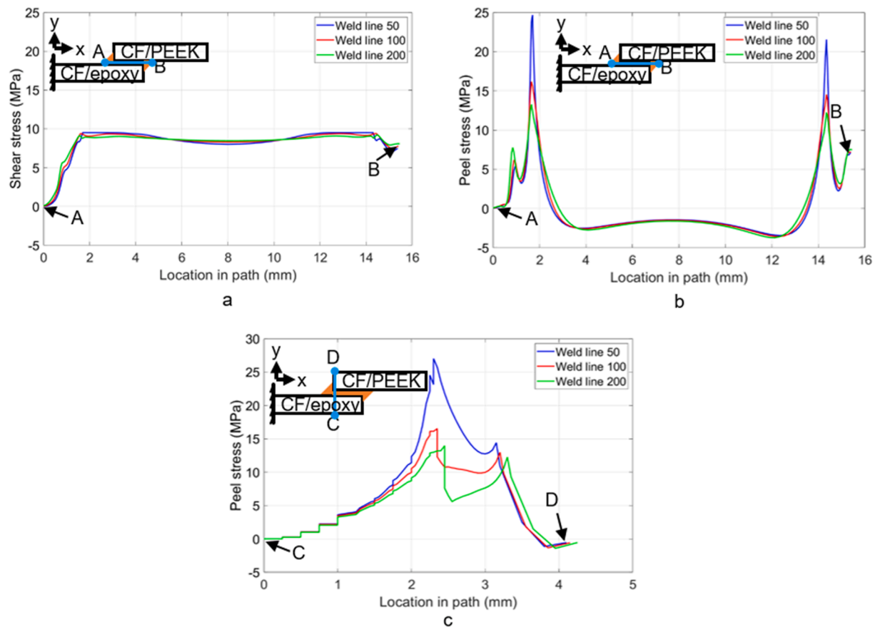
Fig. 6. Stresses obtained from the FE-model. a) Shear stresses along the AB path, b) peel stresses along the AB path and c) peel stresses along the CD path. (For interpretation of the references to color in this figure legend, the reader is referred to the web version of this article.)
