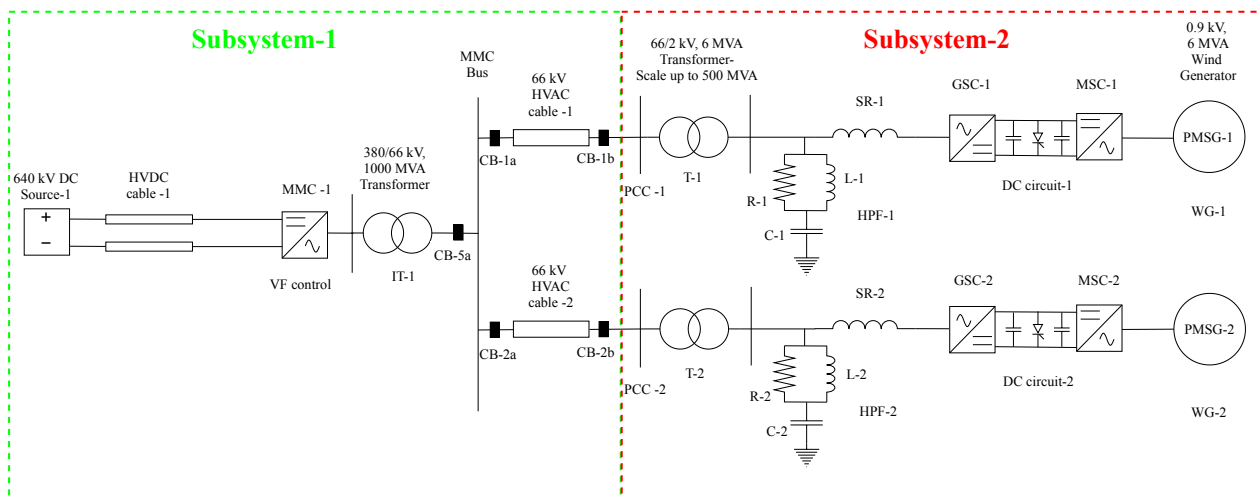
Figure 4. OWF-1 and OWF-2 connected in parallel to MMC-1.
