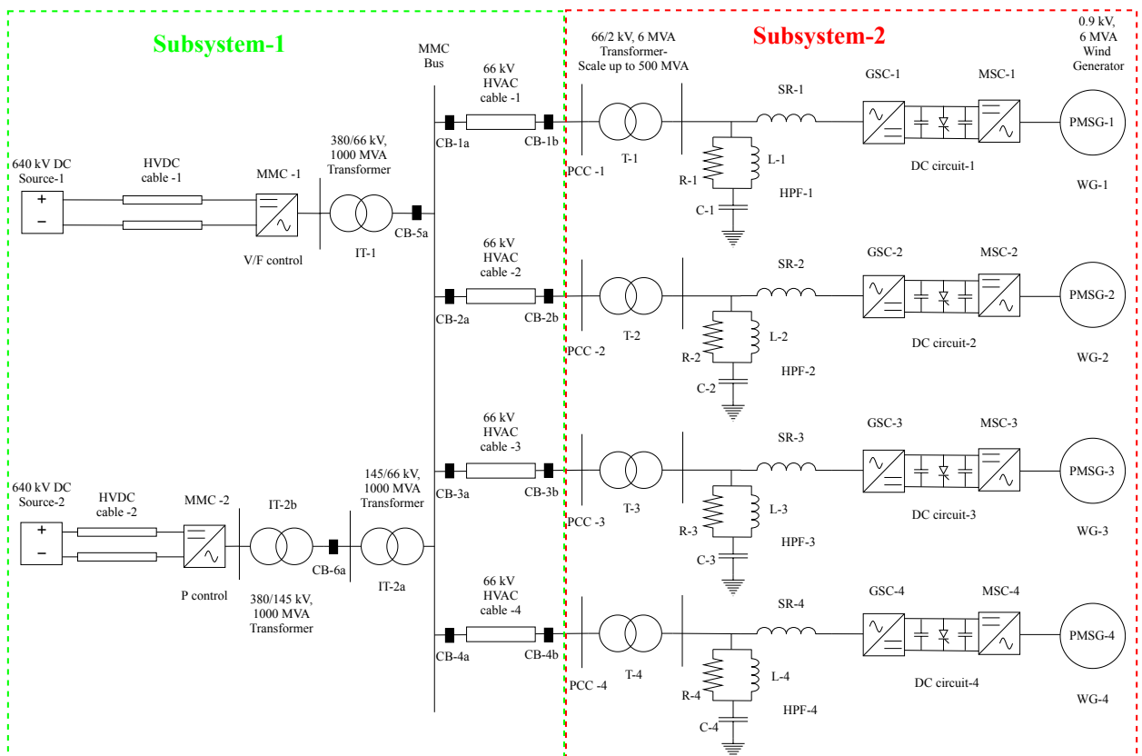
Figure 5. Single line diagram of 2 GW, 66 kV HVAC offshore network connected to 2 × 1 GW HVDC links with offshore converter stations in RSCAD.
