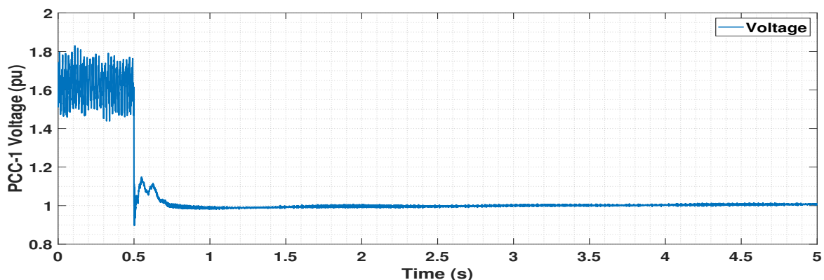
Figure 20. Voltage in p.u. at PCC-1 upon connecting OWF-1 with 50 MW generation to the network.
