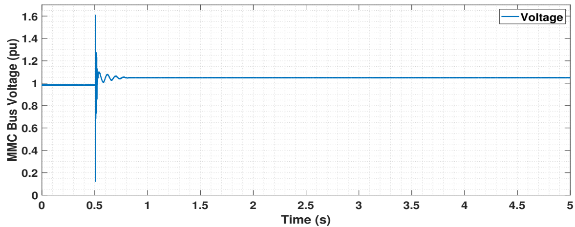
Figure 17. Voltage at MMC bus upon charging of cable-1.
