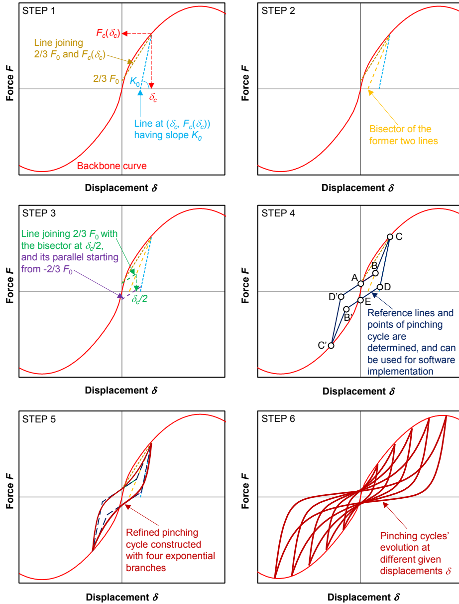
Fig. 9. Procedure for the determination of the pinching cycles from the analytical backbone curve.
