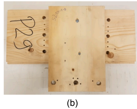
Fig. 3. Samples prepared for the tests on screws fastening the plywood panels to the existing sheathing: schematic description (a) and example of specimen (b).
