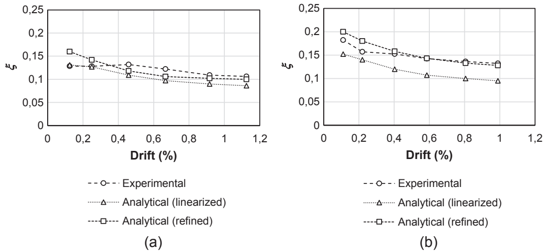
Fig. 13. Example of comparison, for (a) a floor (DFpar-2s) and (b) a roof sample (DRpar-5s), between the analytically predicted equivalent damping ratio (adopting both the linearized and the refined pinching cycle) and the one calculated in [27] from the tests presented in [11].
