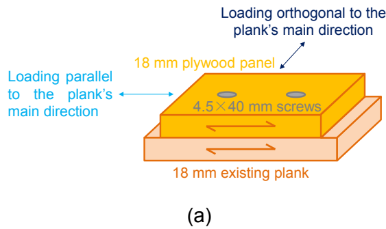
Fig. 3. Samples prepared for the tests on screws fastening the plywood panels to the existing sheathing: schematic description (a) and example of specimen (b).
