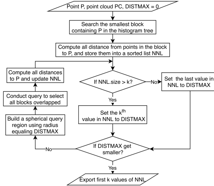
Figure 11. Execution path of k NN using HistSFC
