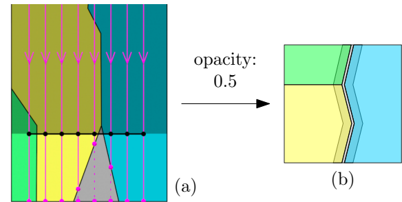
Figure 7. The real representation when drawing semi-opaquely without using a framebuffer.
