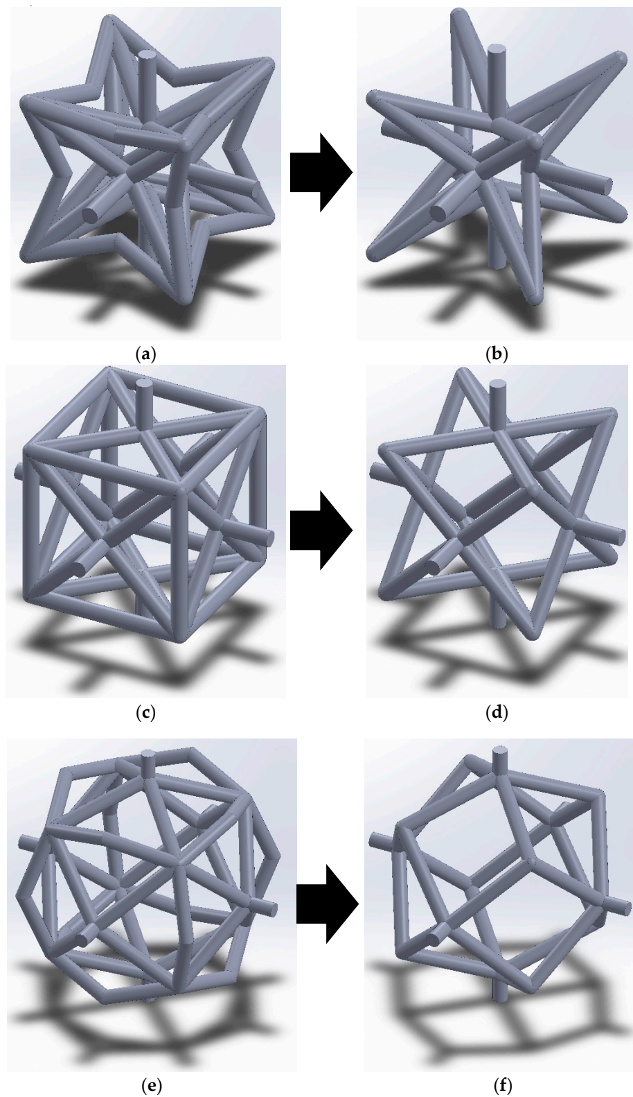
Figure 15. Generic geometry of the unit cell with positive (top), zero (middle), and negative (bottom) values of \theta and \varphi for general unit cell (left column) and lightened unit cell (right column): (a) general re-entrant; (b) lightened re-entrant; (c) general zero Poisson's ratio; (d) lightened zero Poisson's ratio; (e) general convex; and (f) lightened convex unit cells.
