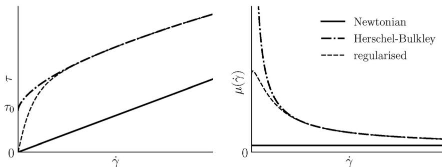
Fig. 1 Shear stress \tau = \mu(\dot{\gamma})\dot{\gamma} and apparent viscosity as a function of the shear rate for Newtonian and Herschel-Bulkley models ( n < 1 ). The dashed lines show the effect of the regularization on the Herschel-Bulkley model. The axes are in linear scales.
