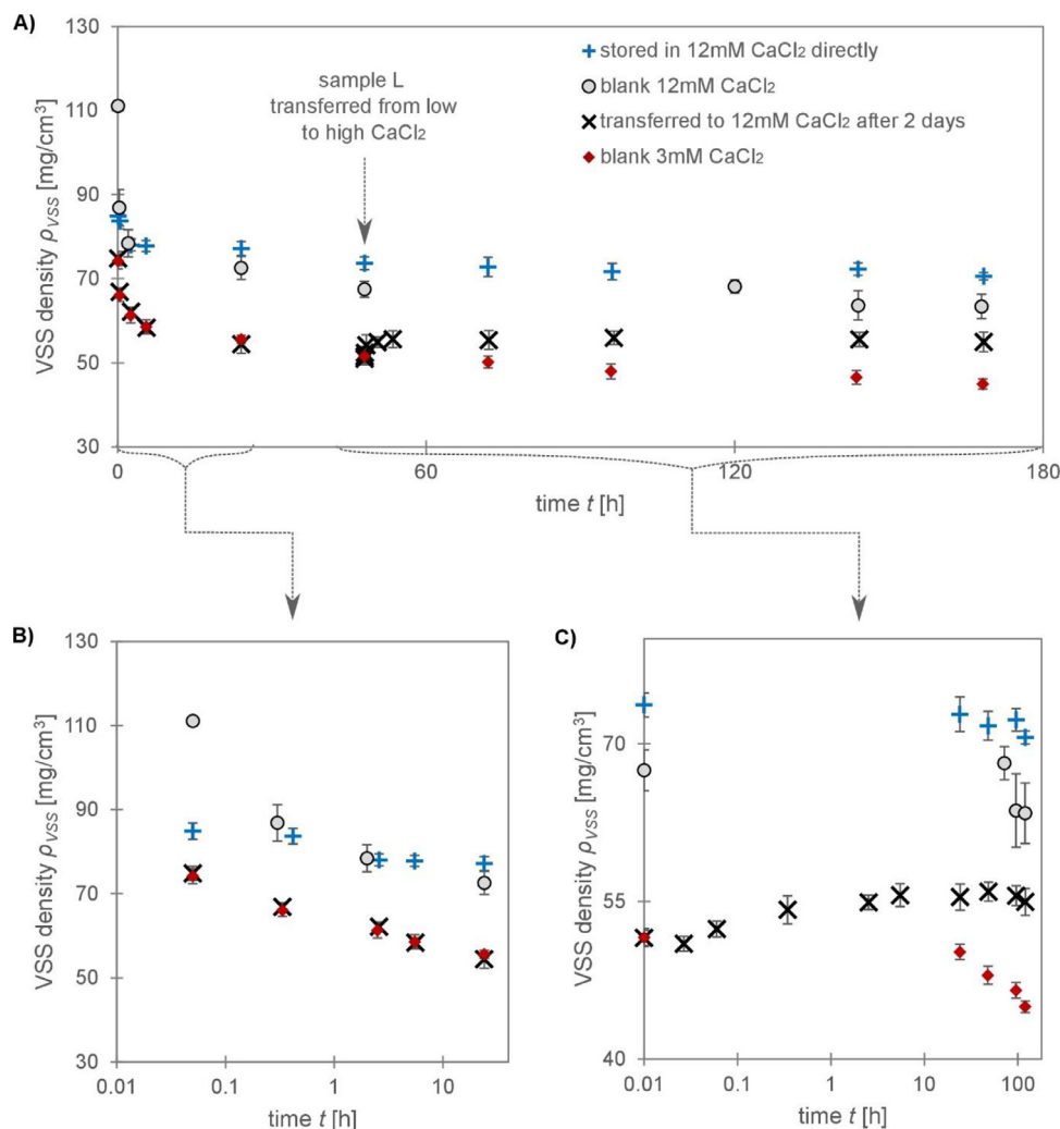
Fig. 5. Comparison of the swelling behaviour of gel layers produced with 3 mM \text{CaCl}_2 and 6 mM KCl and subsequently stored in 12 mM \text{CaCl}_2 /6 mM KCl (high calcium, sample F, +) and 3 mM \text{CaCl}_2 /6 mM KCl for two days and then transferred to 12 mM \text{CaCl}_2 /6 mM KCl (low calcium, sample L, x). For comparison, blanks produced and stored with either high (circle) or low (diamond) calcium concentration are shown. A) shows the whole range of the experiment, B) zoomed in on the first two days and C) zoomed in on the swelling after transfer to the higher calcium concentration after two days. Since those were single experiments, the error bars show the standard deviation over 4 samples only for the high blank.
