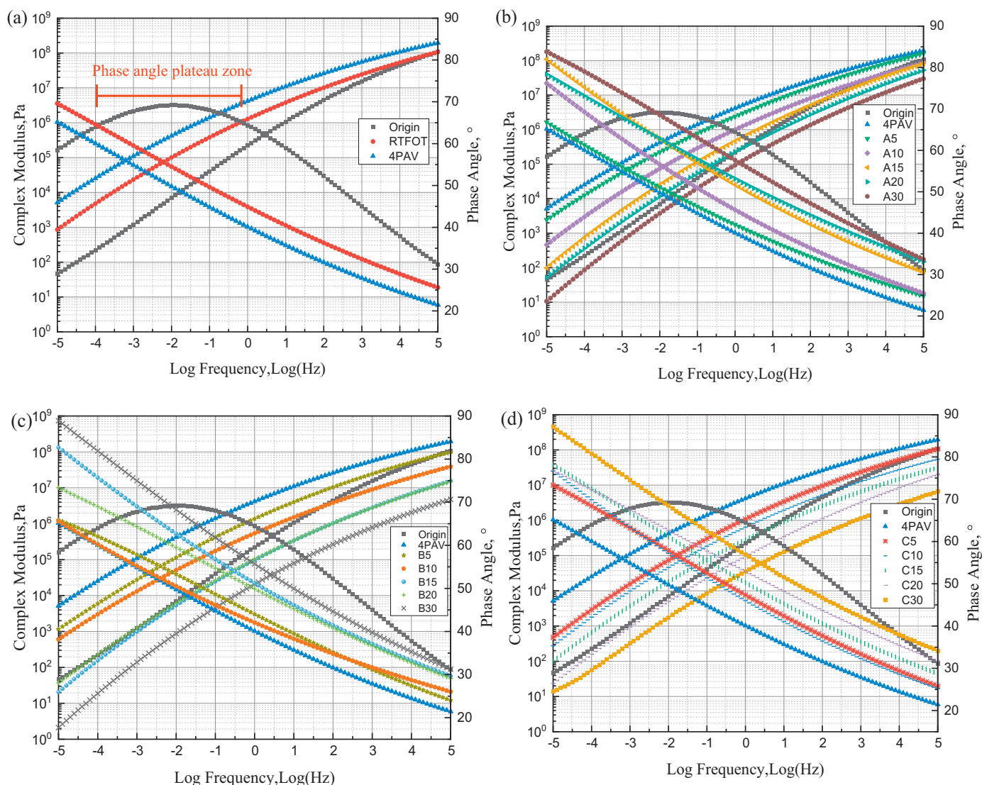
Fig. 3. Complex modulus and phase angle master curve of origin, aged and rejuvenated PMB binders at a reference temperature of 30 °C, (a) origin and aged PMB, (b) rejuvenated bitumen with Rej-A; (c) rejuvenated bitumen with Rej-B; (d) rejuvenated bitumen with Rej-C.
