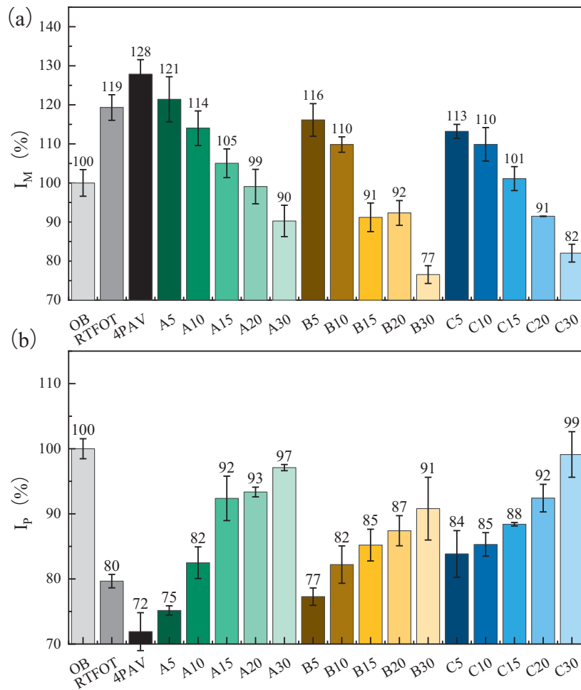
Fig. 4. Complex modulus index and phase angle index of origin, aged and rejuvenated PMB binders, (a) complex modulus index; (b) phase angle index.
