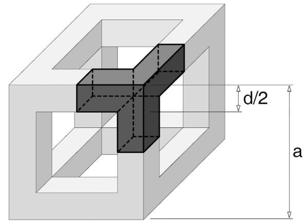
Fig. 13. Model for quantification of parameters of fibril structure of the bitumen microstructure (d: average fibril diameter; a: average space between two adjacent fibrils) [43].
