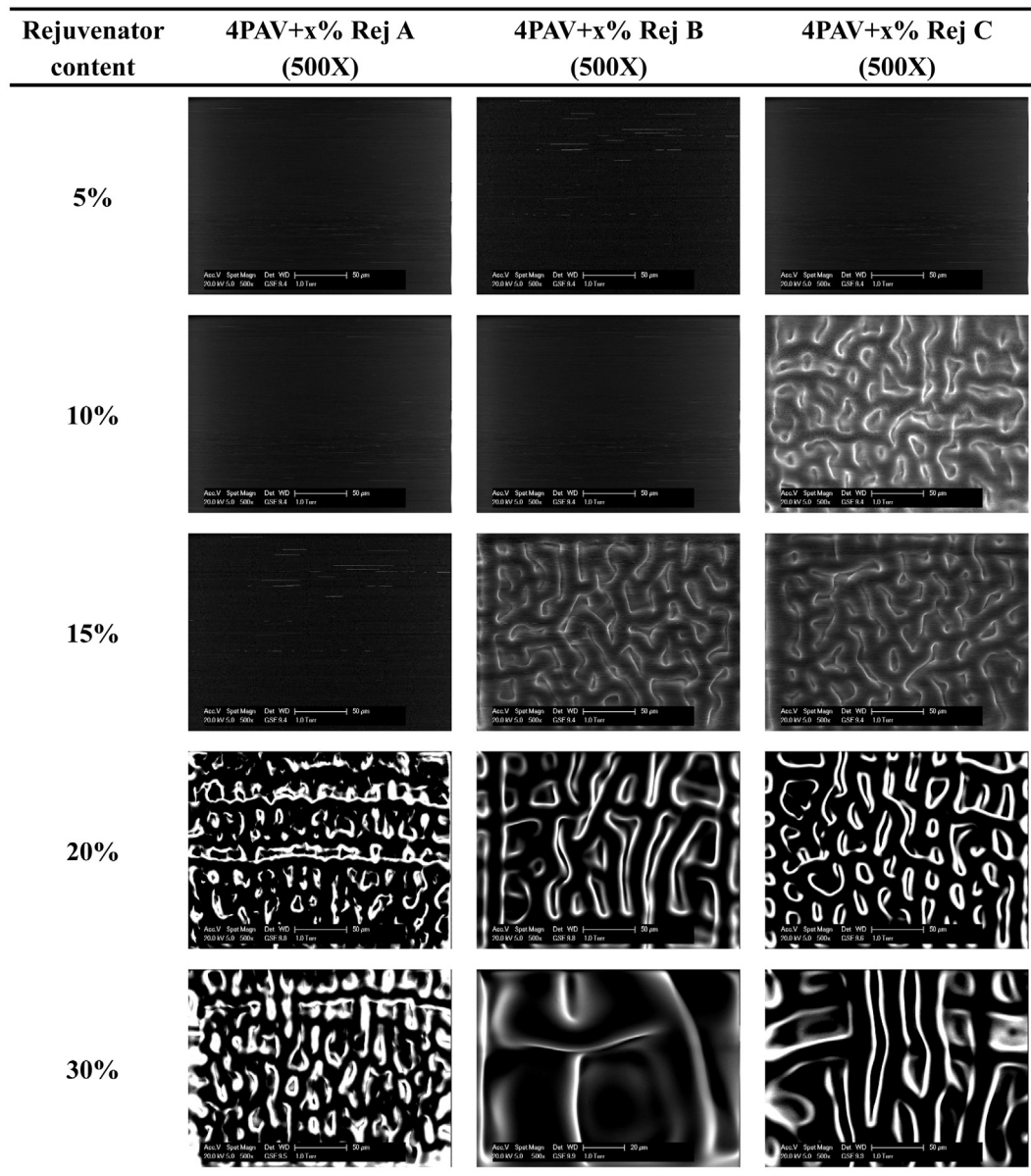
Fig. 9. Microstructures visualized by ESEM for 4PAV aged PMB binder with different types and content of rejuvenator (Illumination time:20 min, Magnification: 500×).
