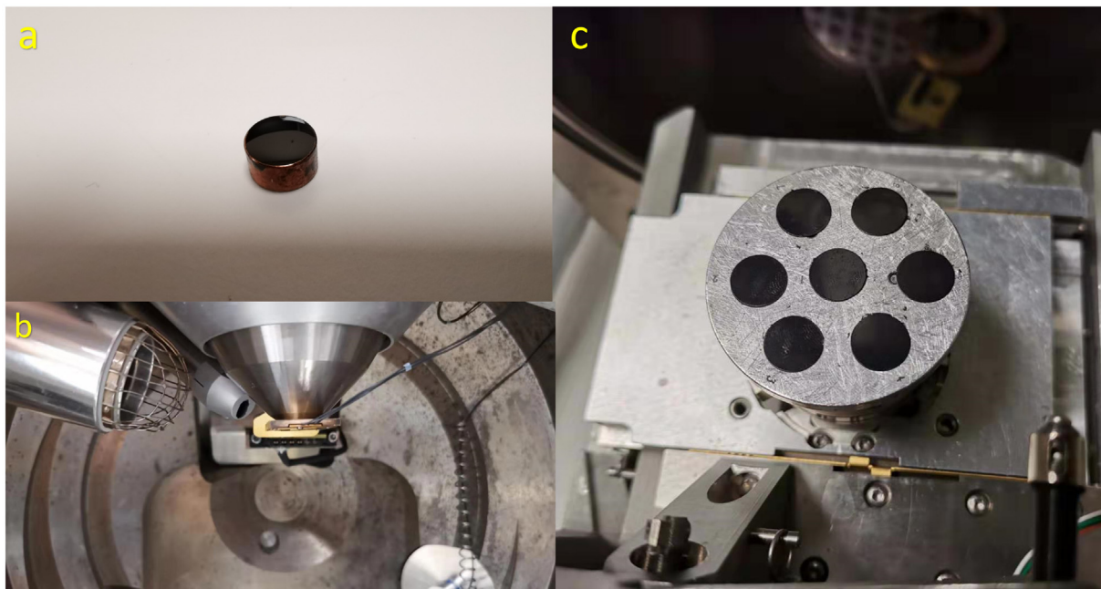
Fig. 2. ESEM device and bitumen sample, (a) bitumen sample, (b) detector and electron gun and (c) ESEM sample stage.
