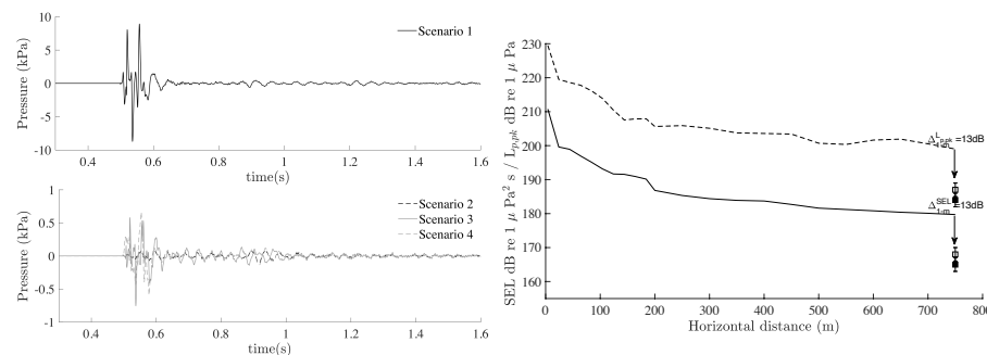
Figure 8. Prediction of the noise from the pile driving: (left) computed time histories of the pressure in the water at various radial distances at 2 m above the seabed, in which scenario 1 indicated by the black solid line; scenario 2 indicated by the black dashed line; scenario 3 indicated by the gray solid line; scenario 4 discussed in Section 6.2 indicated by the gray dashed line; and (right) comparison of SEL and L_{p,pk} at 750 m radial distance from the pile and 2 m above the seabed with the comparison between the scenario 1 and arithmetic mean measured data.
