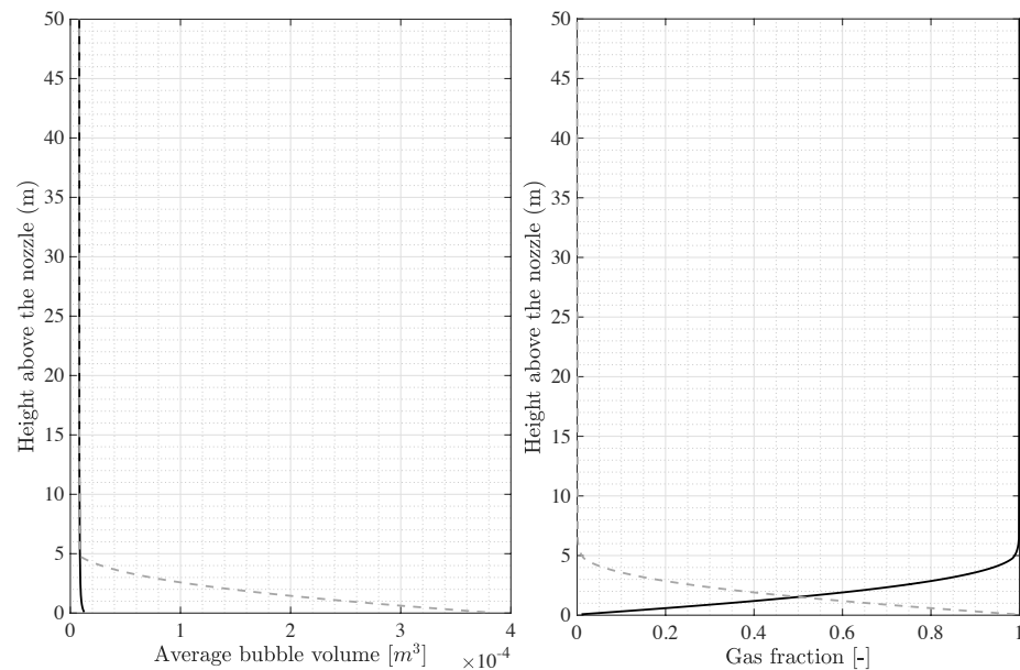
Figure 6. Computed depth-dependent variables for the case of the air flow rate being 0.024 \text{ m}^3/\text{s} : (left) the arithmetic mean bubble volumes and the (right) gas fraction ratio ( \frac{\epsilon_{gmi}}{\epsilon_{gm1} + \epsilon_{gm2}} ) varying over the depth, in which the black solid line indicates the results for small bubbles and gray dashed line represents the results for large bubbles.
