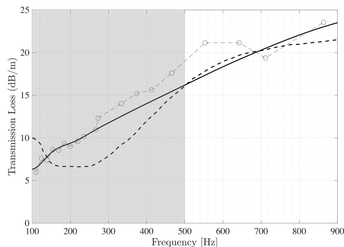
Figure 7. Comparison of the transmission loss between the modeling results (the black solid line) and the data from the measurement [42] (the line with circles) and the numerical air bubble curtain model [27] without the assumption of the bubble size distribution coefficients (the black dashed line). The light gray area indicates the frequencies of interest in offshore pile driving (<500 Hz).
