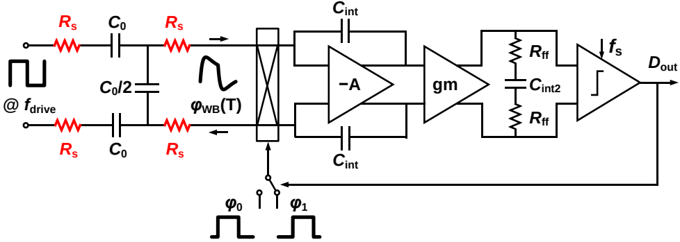
Figure 3.16: Simplified circuit diagram of the first WB sensor implementation.
