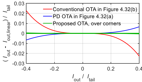
Figure 4.36: Relative nonlinearity with different OTA structures.
