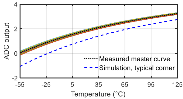
Figure 4.18: Measured and simulated sensor output vs. temperature.
