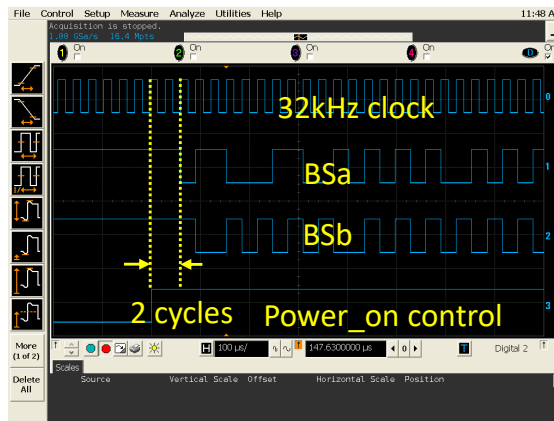
Figure 5.12: Measured BS outputs of a chip around the rising edge of power-on control.
