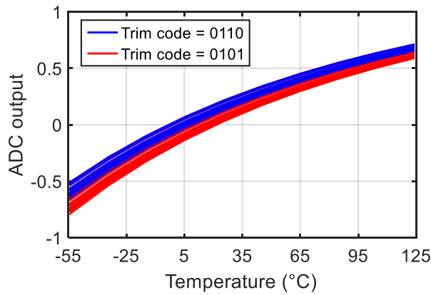
Figure 4.27: Sensor characteristic with different trimming codes.
