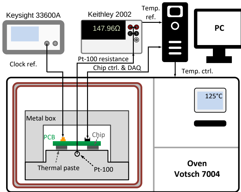
Figure A.2: Test setup for temperature sensor characterization.
