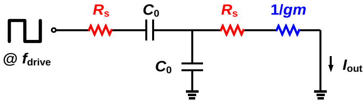
Figure 3.18: Additive resistance on the output resistor of Wien bridge sensor when using an OTA-based first stage.
