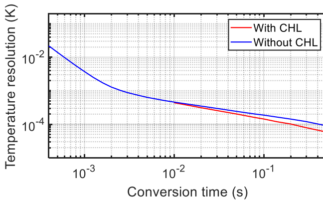
Figure 3.42: Resolution vs. conversion time over a 1s period, with/without system-level chopping.
