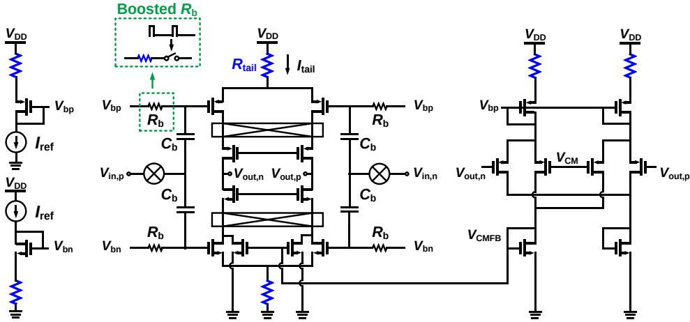
Figure 4.35: Simplified schematic diagram of the linearized OTA, including the biasing generation and CMFB circuit.
