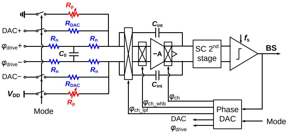
Figure 5.15: Simplified circuits diagram of the LPF/WhB readout circuit.
