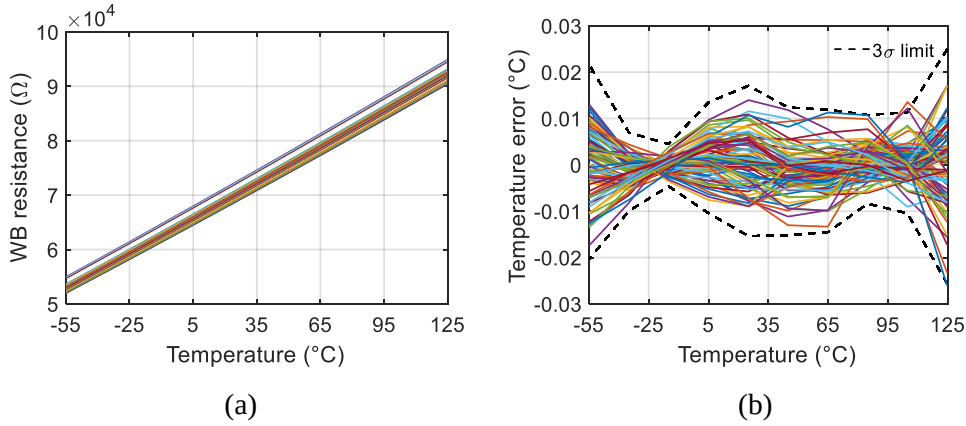
Figure 3.43: (a) Extracted sensor resistance and (b) sensor inaccuracy after a 1st-order fit and systematic non-linearity correction.
