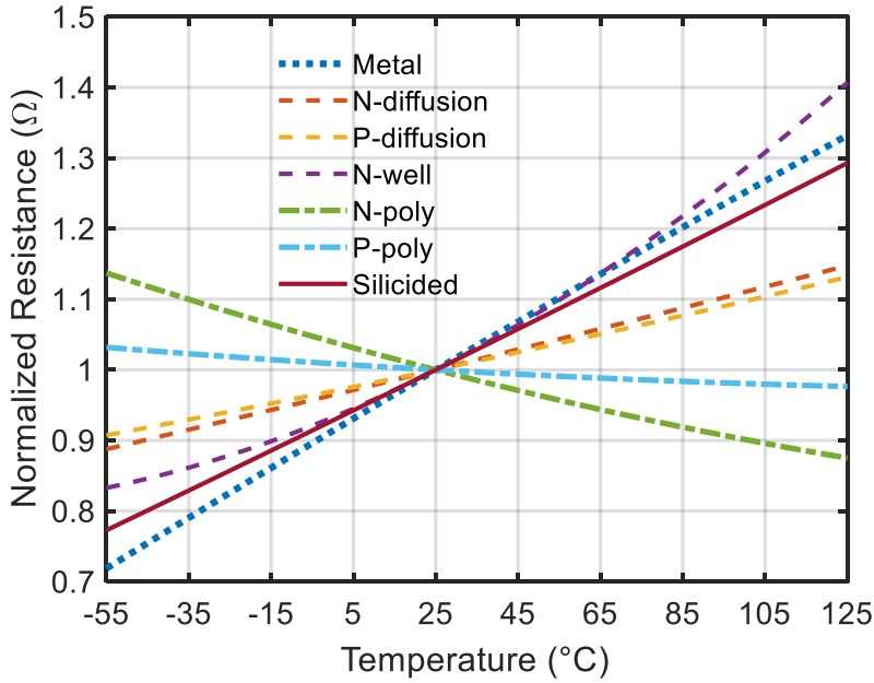
Figure 1.10. Temperature characteristics of different resistors in a standard 0.18\mu\text{m} CMOS technology.
