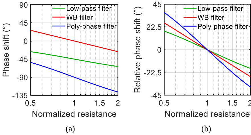
Figure 2.8: (a) Phase shift and (b) relative phase shift of different RC filters as a function of normalized resistance.
