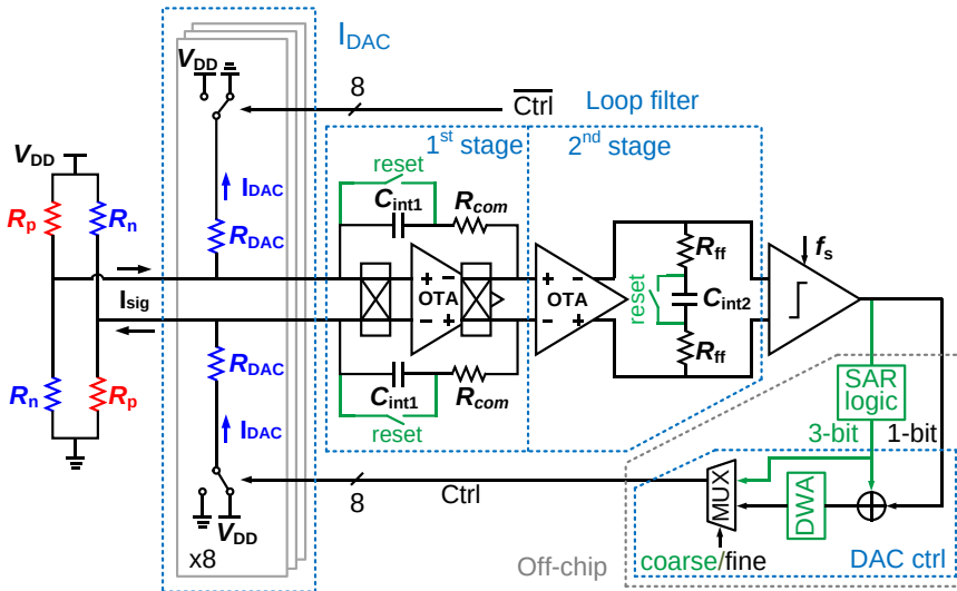
Figure 4.12: Circuit diagram of the zoom CT \Delta\Sigma -ADC.
