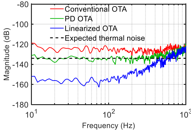
Figure 4.38: Simulated \Delta\Sigma bitstream spectrum without noise using the same I_{\text{tail}} but different OTA configurations.
