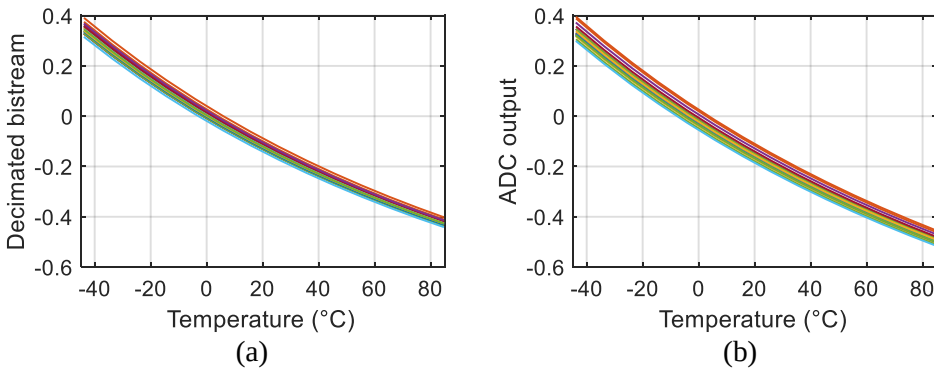
Figure 4.5: Output vs. temperature of (a) s-p-poly/n-poly WhB sensors and (b) s-p-poly/p-poly WhB sensors.
