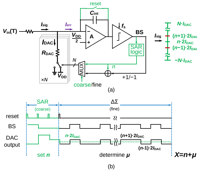
Figure 4.11: (a) Schematic of a static zoom CT \Delta\Sigma and (b) a timing diagram example in case of a 3-bit DAC.
