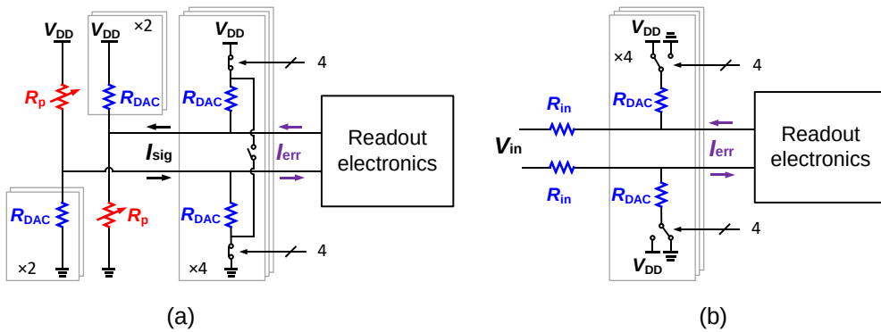
Figure 6.6: (a) Wheatstone bridge front end shown in section 4.6. (b) Input and DAC resistors of a CT \Delta\Sigma -ADC with equivalent input impedance and noise.
