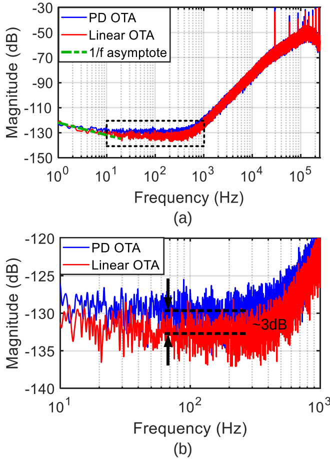
Figure 4.45: (a) Bitstream spectra of the sensor with different OTA configurations (10M samples, Hanning window, 10\times averaging) and (b) a zoomed-in plot from 10Hz to 1kHz.
